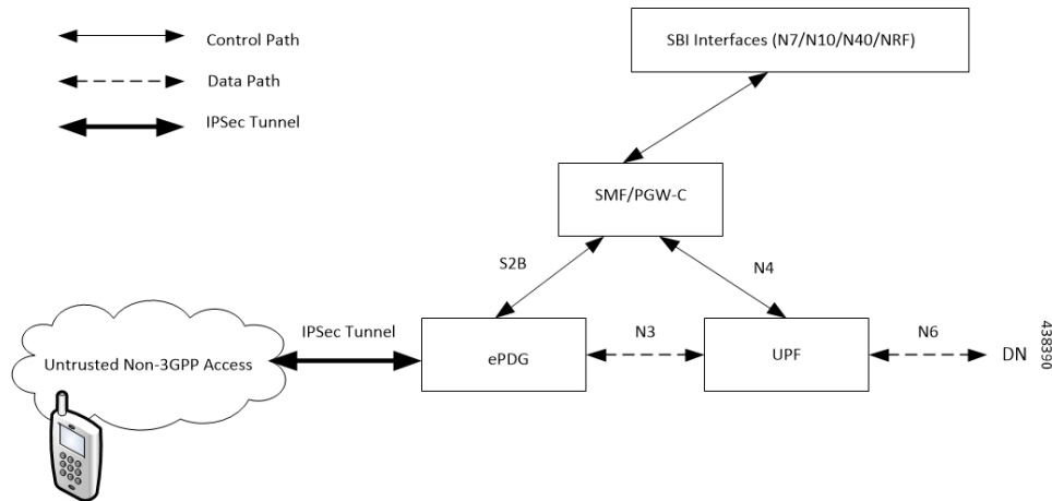
Figure 1: VoWiFi Architecture
