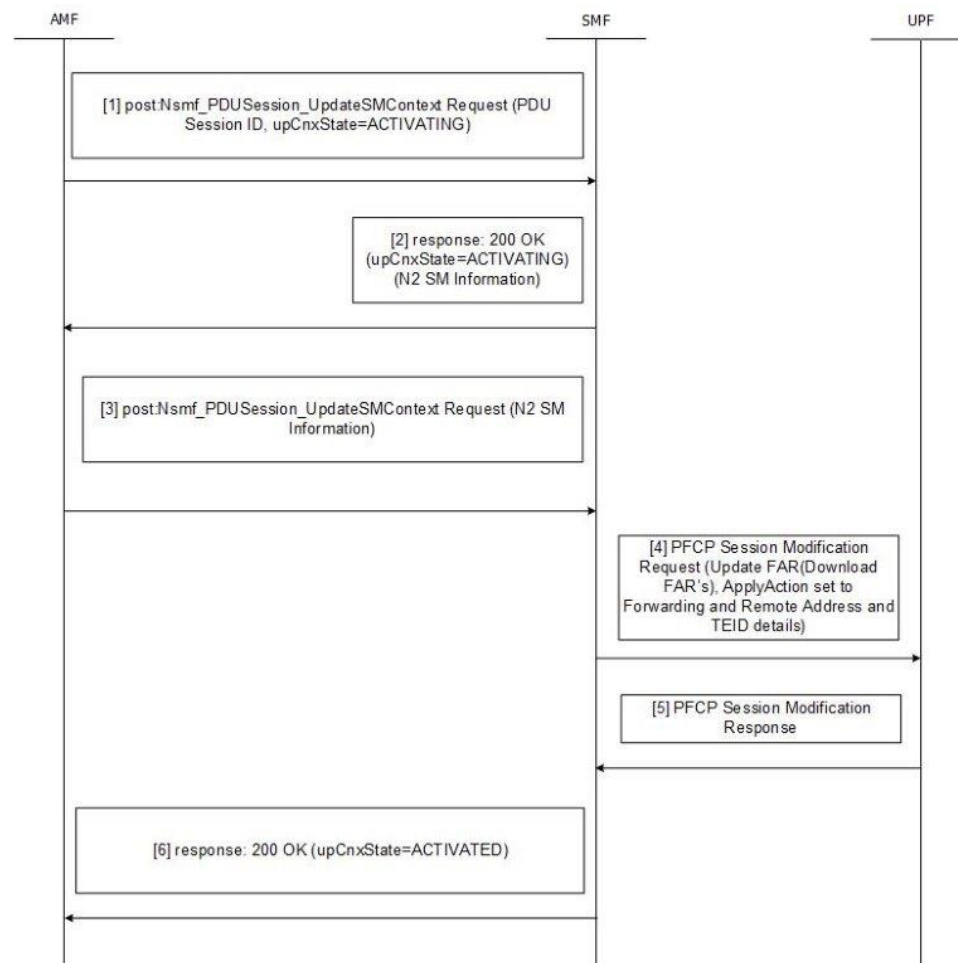
Figure 1: Idle to Active Transition (UE-Initiated) Call Flow
