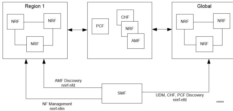
Figure 11: NRF Deployment
