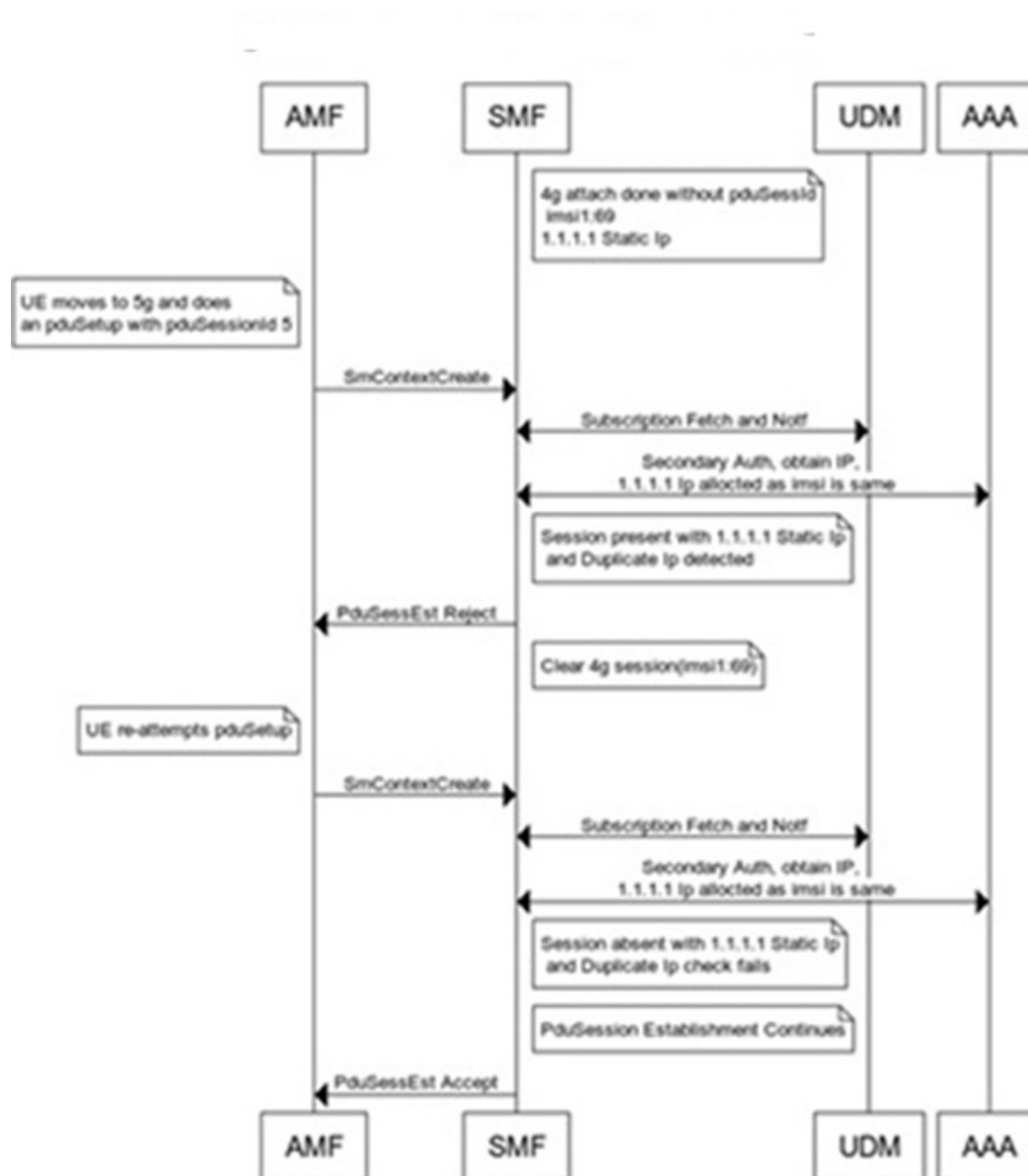
Figure 4: Duplicate static IP detection
