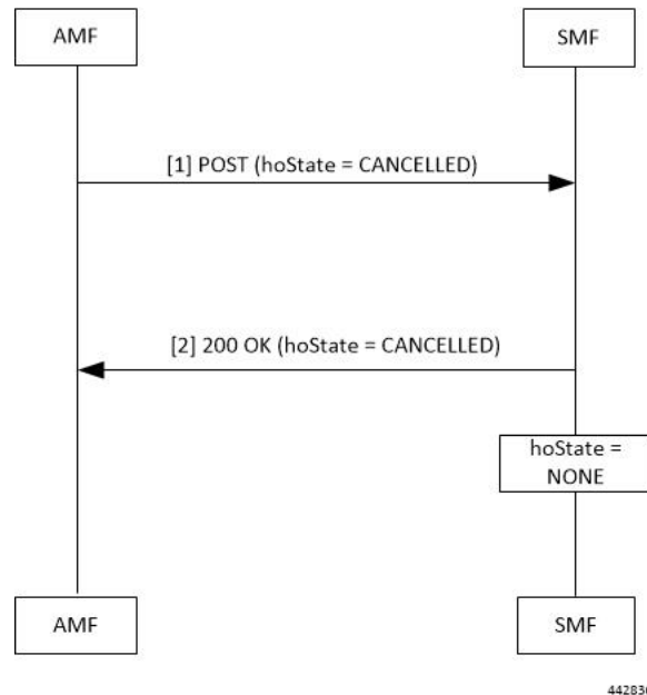
Figure 44: 5GS to EPS Handover Cancellation Call Flow
