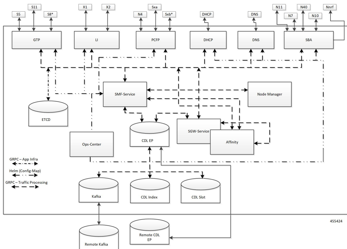
Figure 4: Kubernetes Deployment
