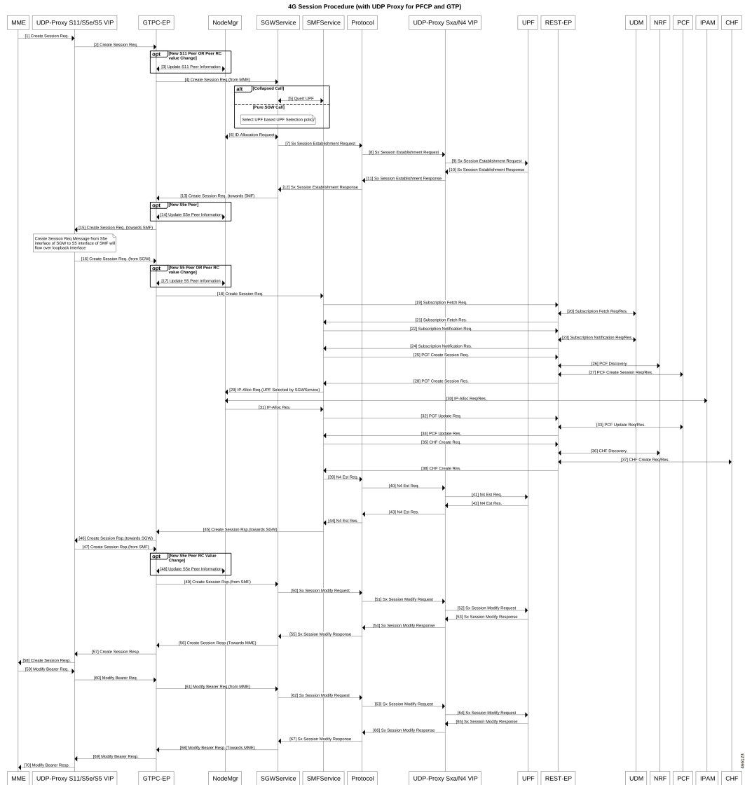
Figure 6: 4G Session Procedure with UDP Proxy for PFCP and GTP
