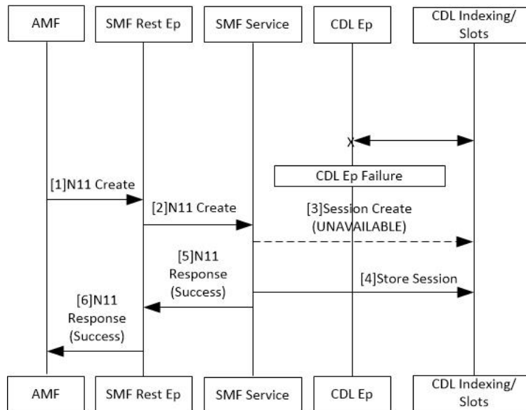
Figure 2: CDL endpoint failure call flow
