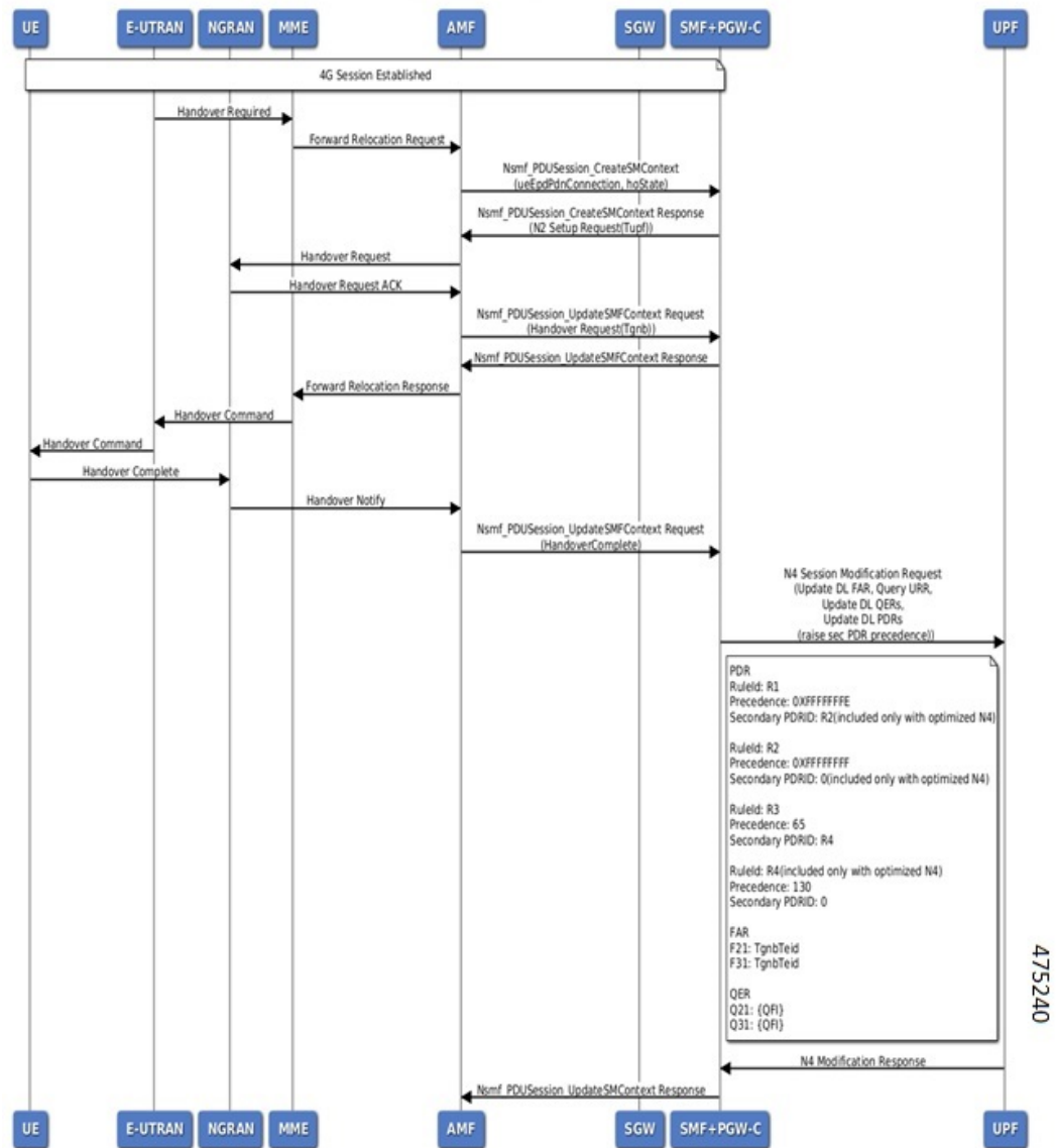
Figure 25: Call Flow for Inter-plmn HO from 4G Roamer to 5G Homer
