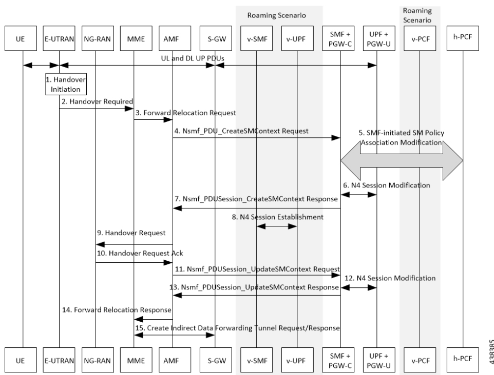
Figure 13: Call Flow for the EPS to 5G Handover Using the N26 Interface
