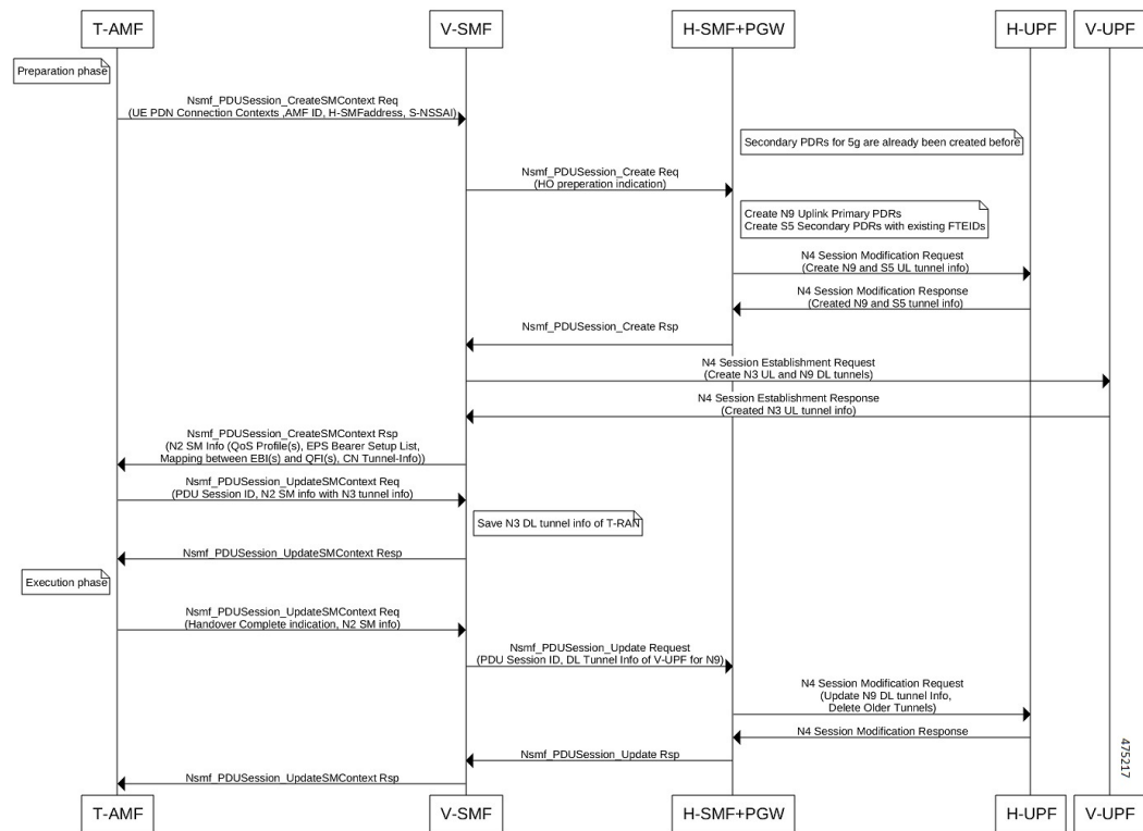
Figure 21: Call Flow for Inter-plmn N26 HO from 4G Homer to 5G Roamer
