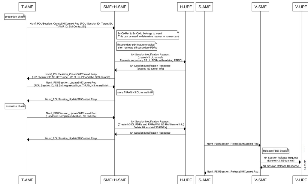
Figure 20: Call Flow for Inter-plmn N2 HO with v-SMF Deletion
