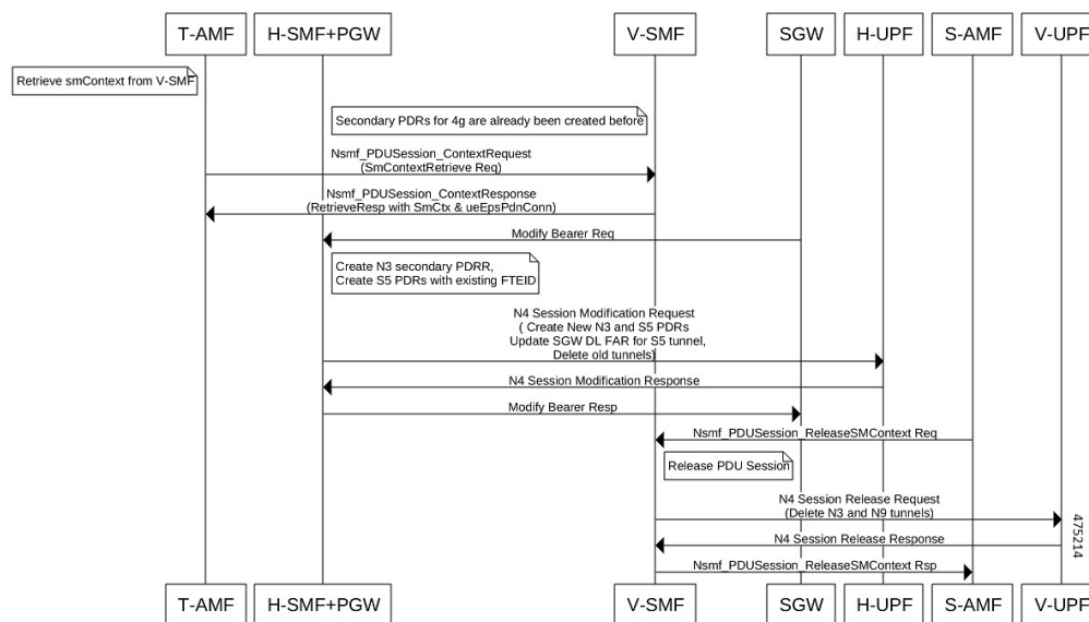
Figure 22: Call Flow for Inter-plmn HO from 5G Roamer to 4G Homer
