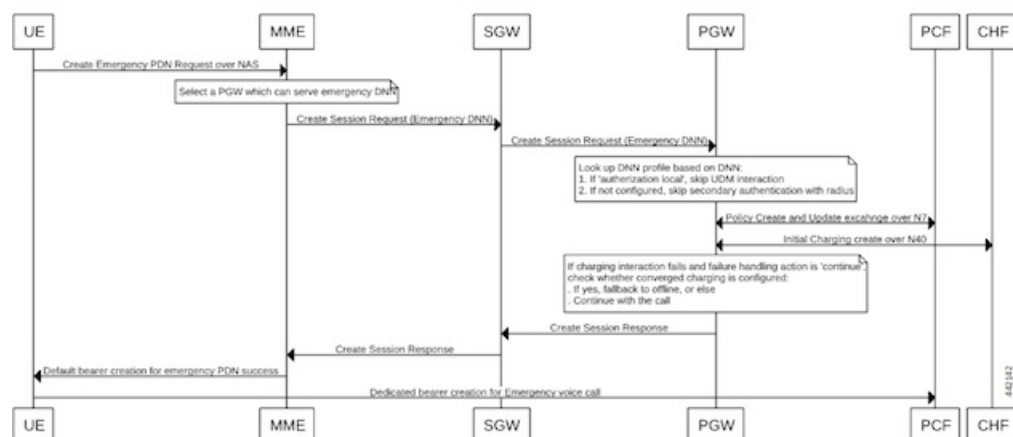
Figure 1: Emergency Session Creation in LTE
