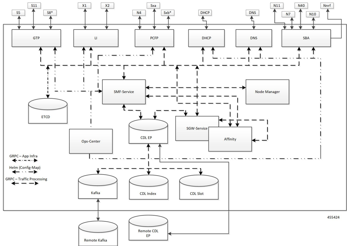
Figure 4: Kubernetes Deployment
