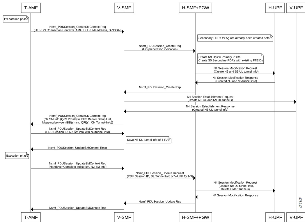
Figure 22: Call Flow for Inter-plmn N26 HO from 4G Homer to 5G Roamer
