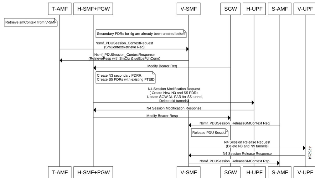
Figure 23: Call Flow for Inter-plmn HO from 5G Roamer to 4G Homer
