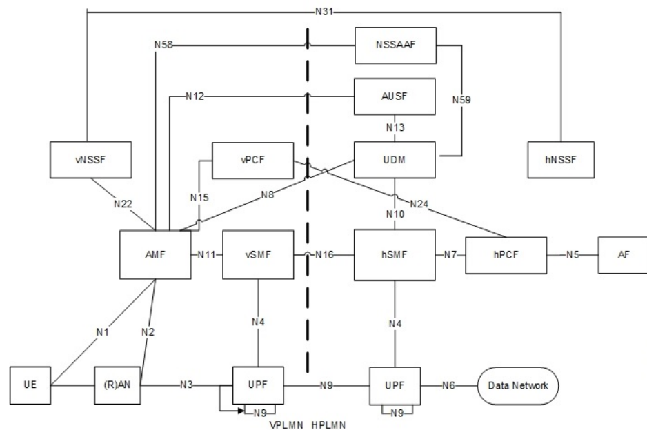
Figure 5: 5G NR HR Roaming Architecture
