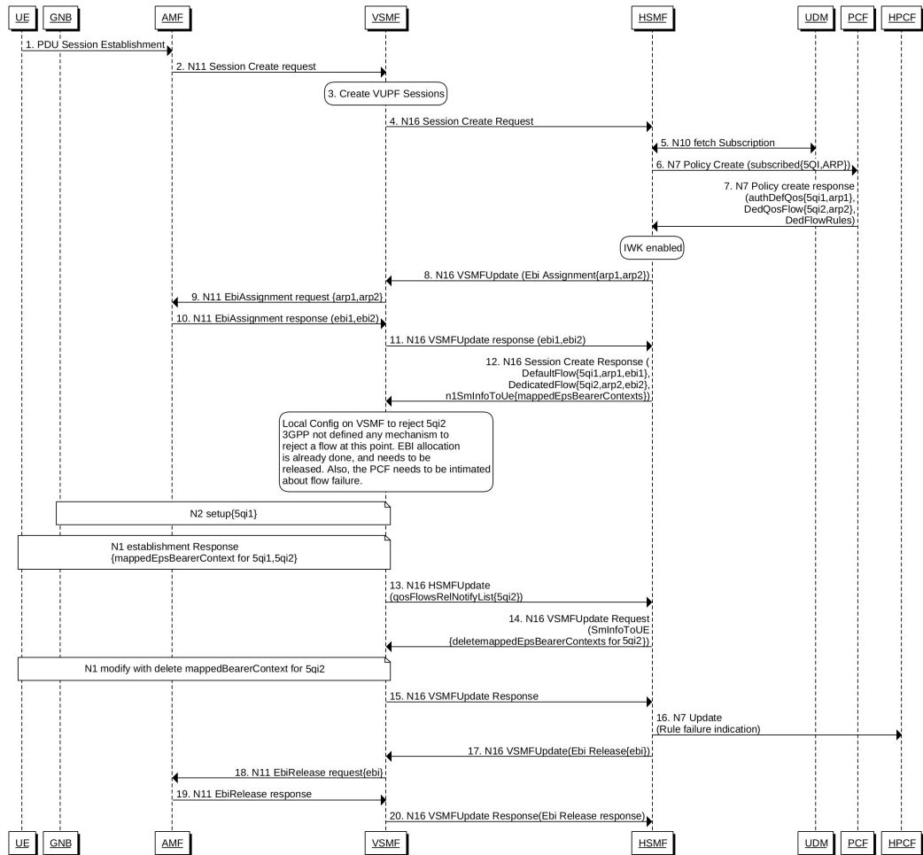
Figure 18: Call Flow for 5QI Rejection During 5G Session Creation
