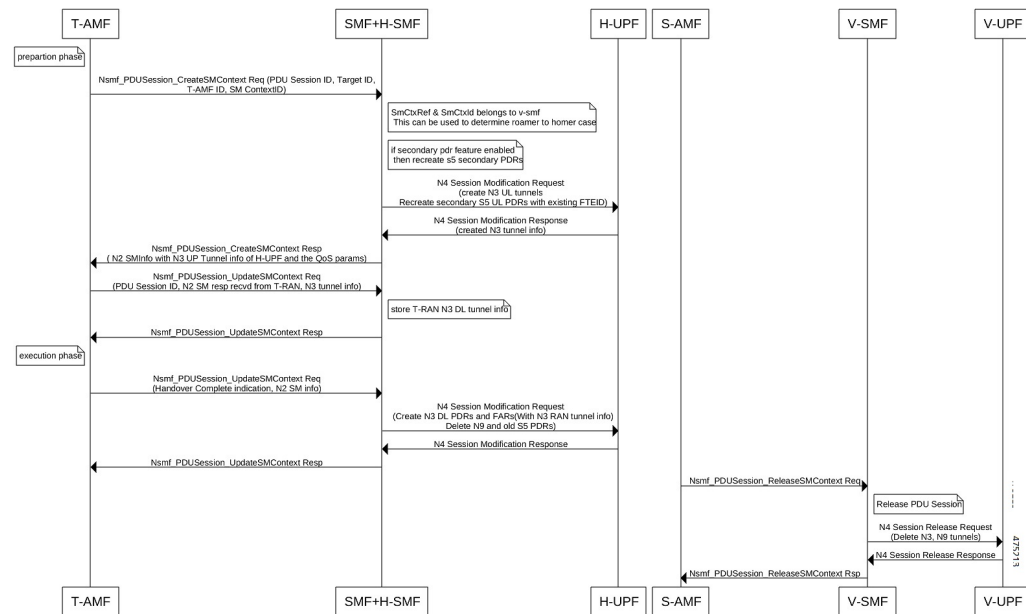
Figure 21: Call Flow for Inter-plmn N2 HO with v-SMF Deletion
