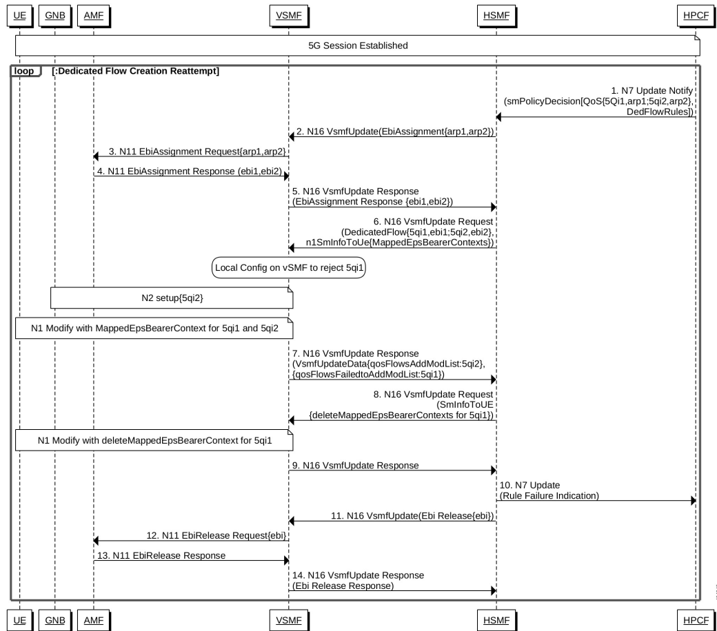
Figure 19: Call Flow for 5QI Rejection During Dedicated Flow Creation
