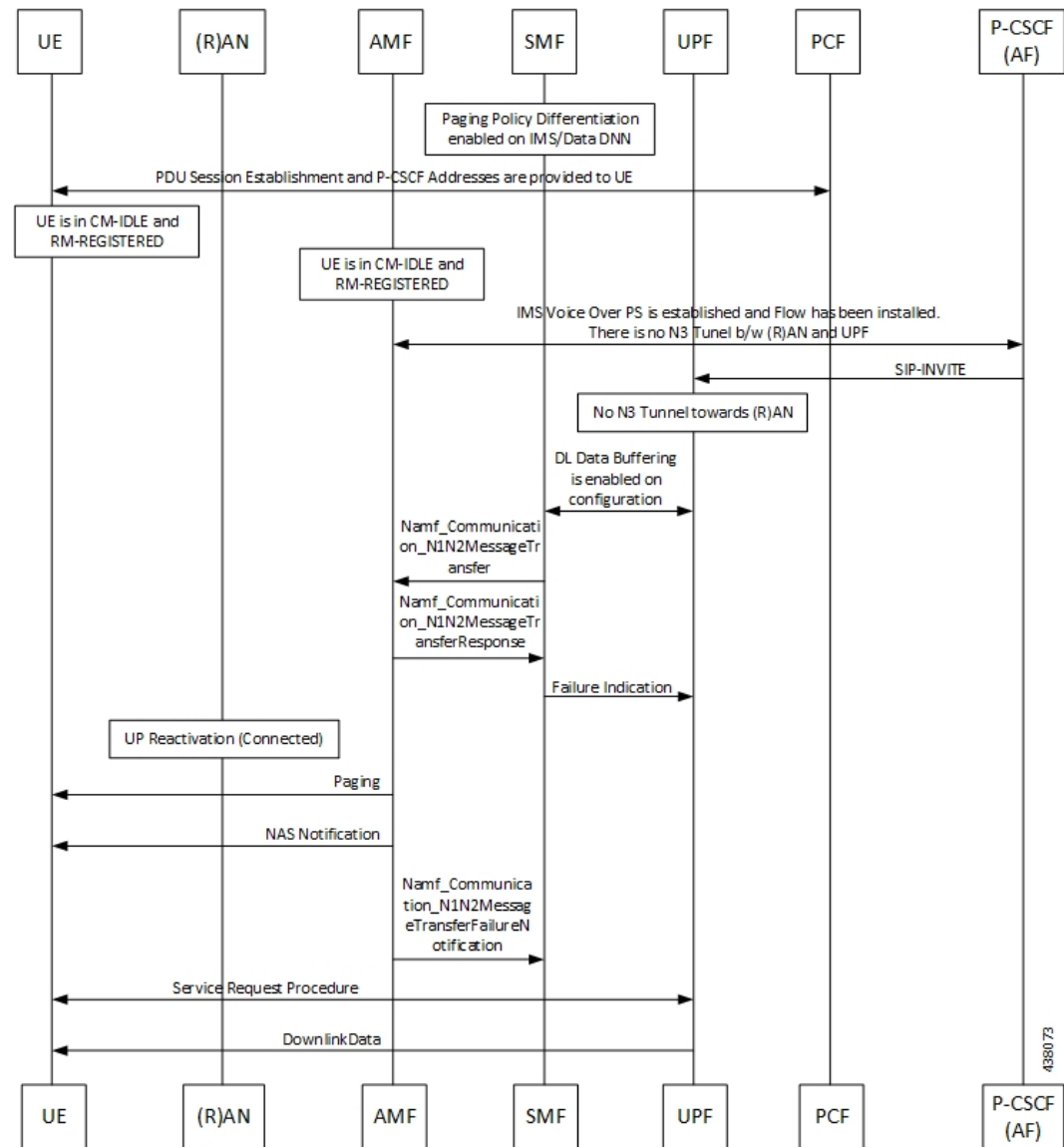
Figure 12: VoNR MT Call Flow for UE in Idle Mode
