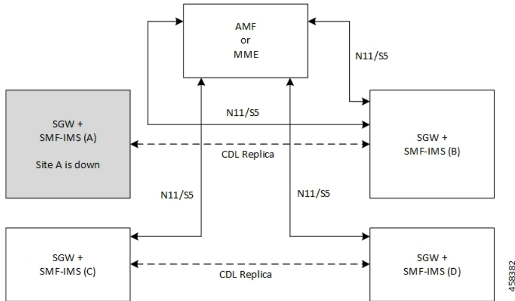
Figure 5: Geo HA for Internal Network Failure
