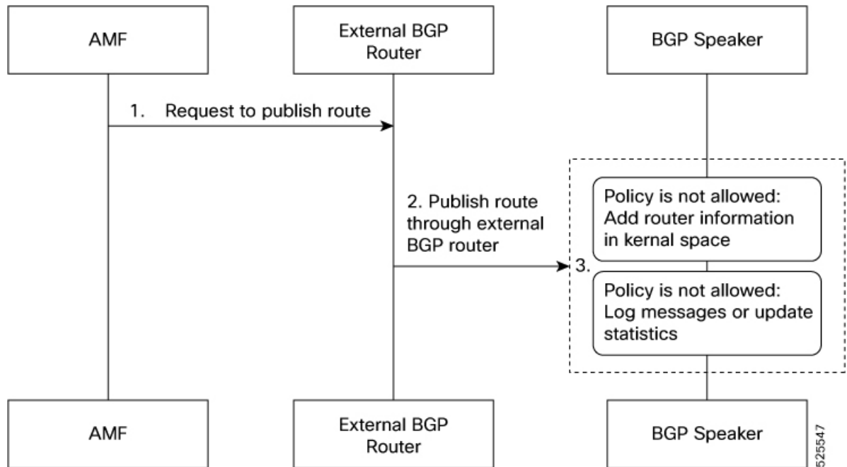
Figure 9: Learn Route for Outgoing Traffic Call Flow
