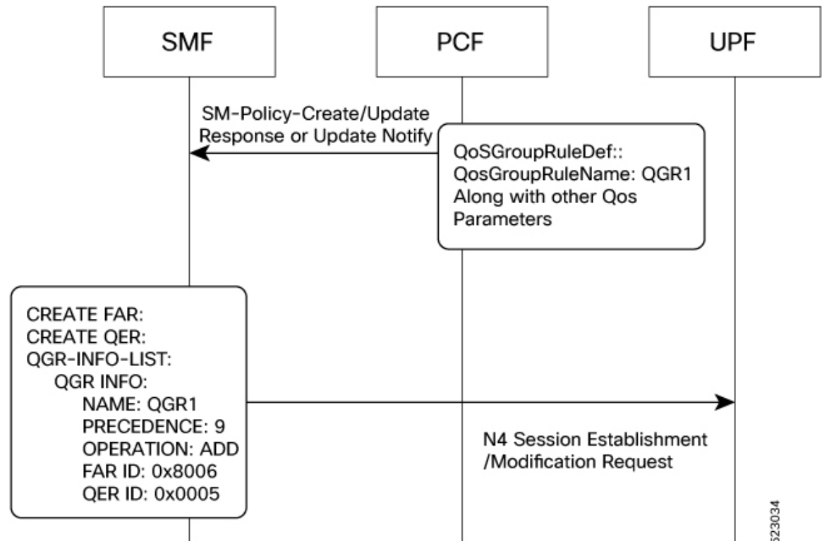
Figure 22: Qos-Group-of-Ruledef Activation Call Flow
