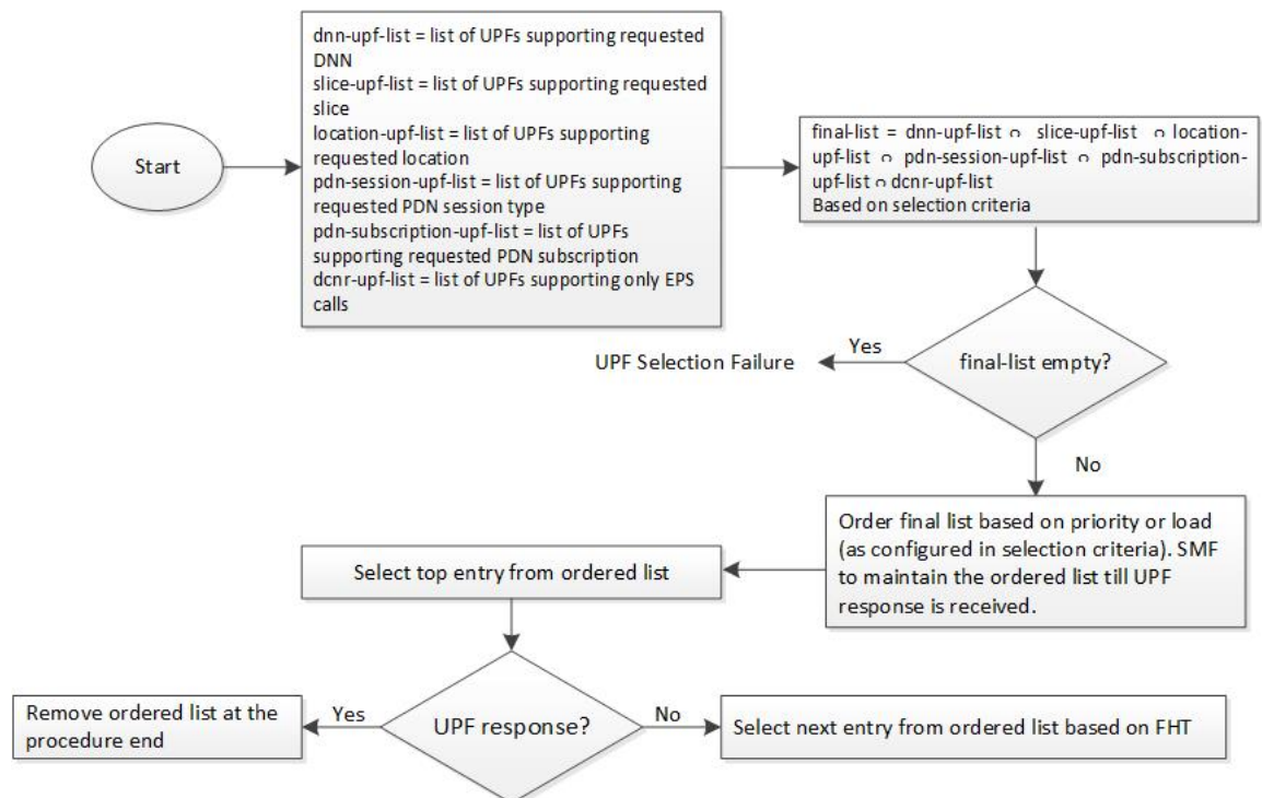
Figure 14: UPF Node Selection Workflow
