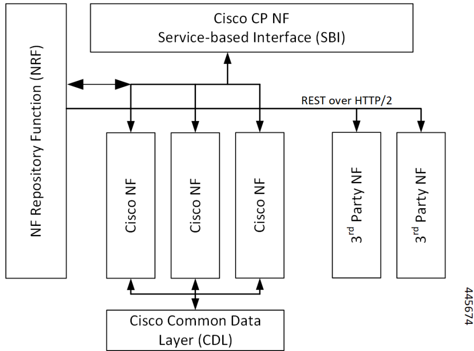
Figure 4: Cisco CP NF Service-based Architecture Support
