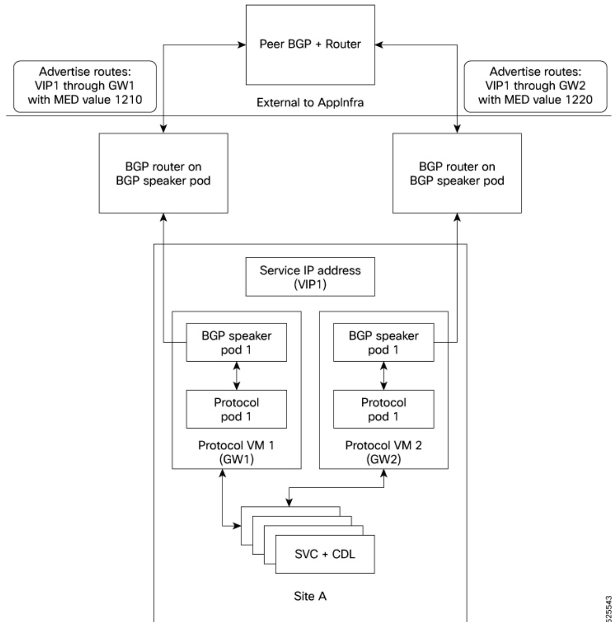
Figure 4: Dynamic Routing for Incoming Traffic in the Active-standby Topology
