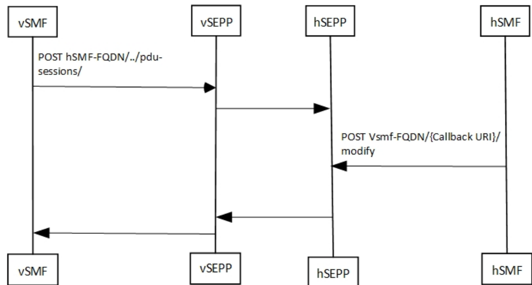
Figure 17: Call Flow with SEPP
