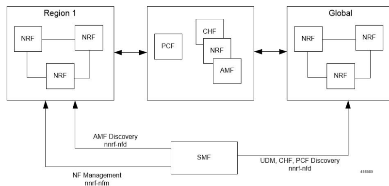
Figure 11: NRF Deployment
