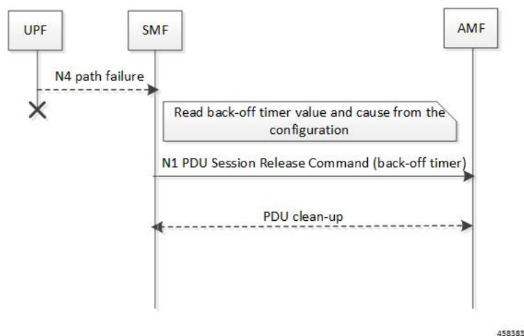
Figure 1: N4 Path Failure Handling Call Flow for Non-roaming Session
