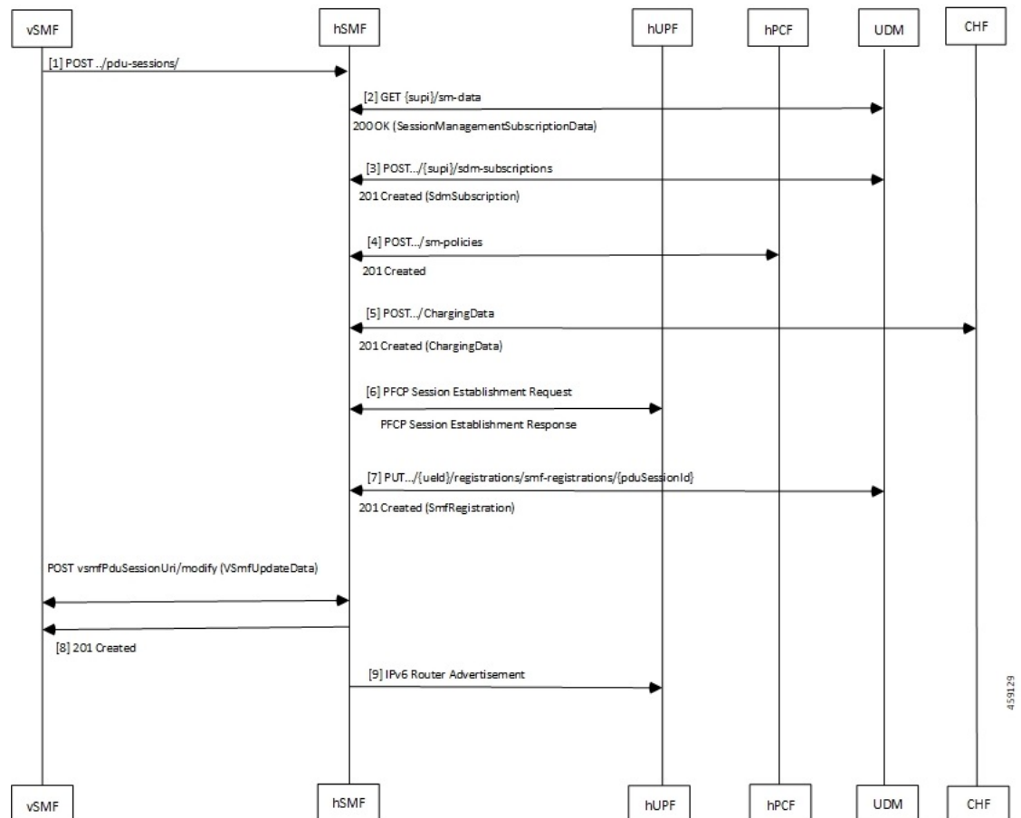
Figure 7: hSMF Create Session Call Flow
