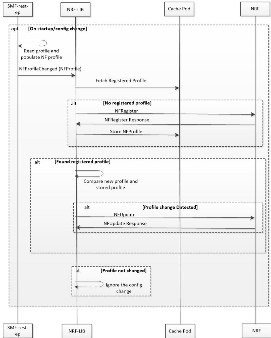
Figure 9: NF Registration and NF Update Call Flow
