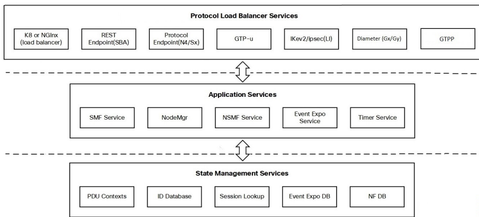
Figure 1: SMF Architecture
