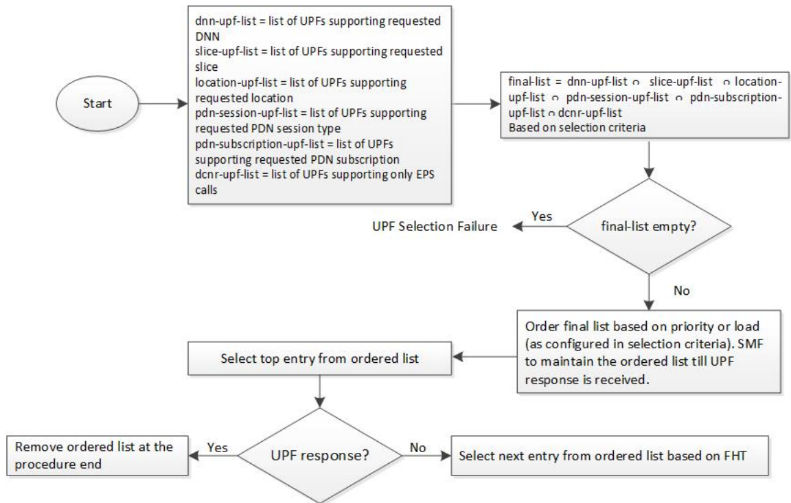
Figure 11: UPF Node Selection Workflow
