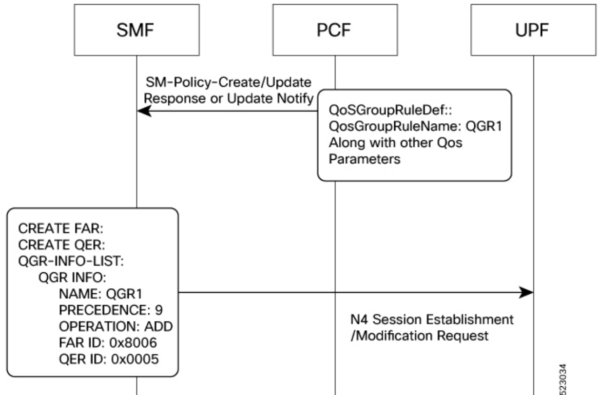
Figure 19: Qos-Group-of-Ruledef Activation Call Flow
