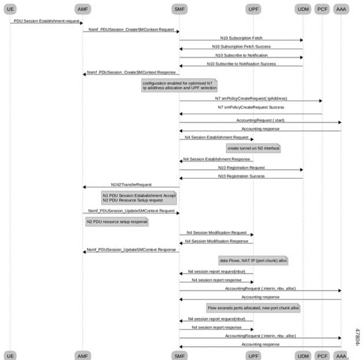
Figure 4: Call Flow for Port Chunk Allocation
