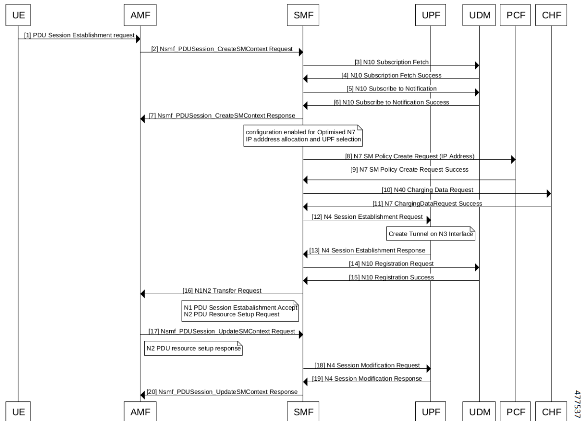
Figure 9: 5G Session Creation with N7 Optimization Call Flow
