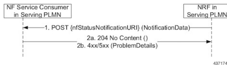
Figure 6: NFStatus Notify Call Flow
