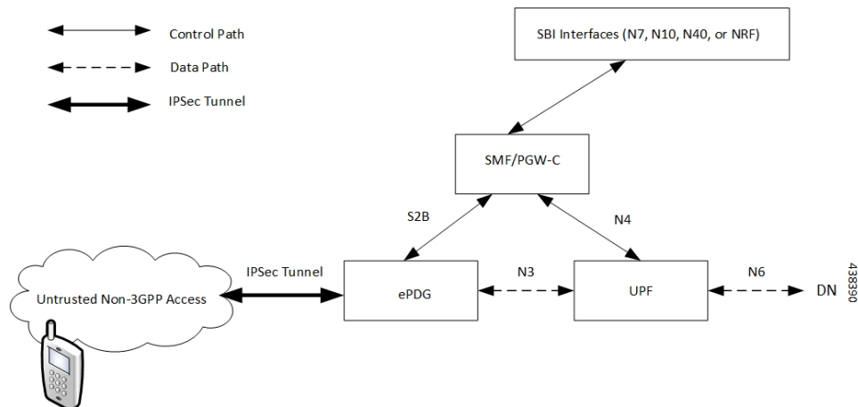
Figure 4: VoWi-Fi Architecture
