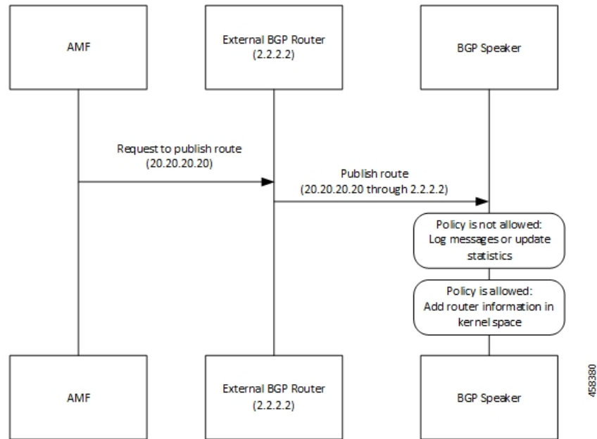
Figure 6: Learn Route for Outgoing Traffic Call Flow
