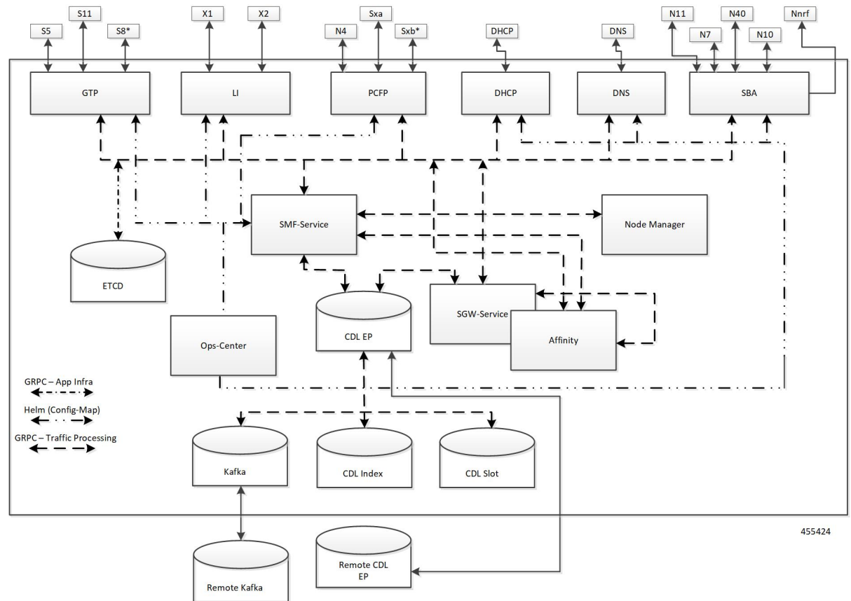
Figure 3: Kubernetes Deployment
