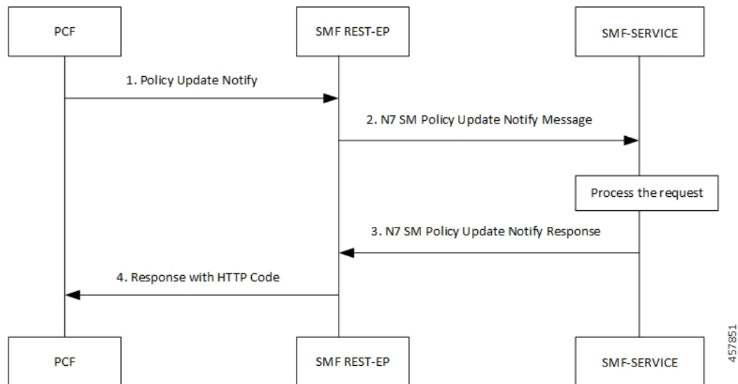
Figure 1: SM Policy Update Notify Service from PCF
