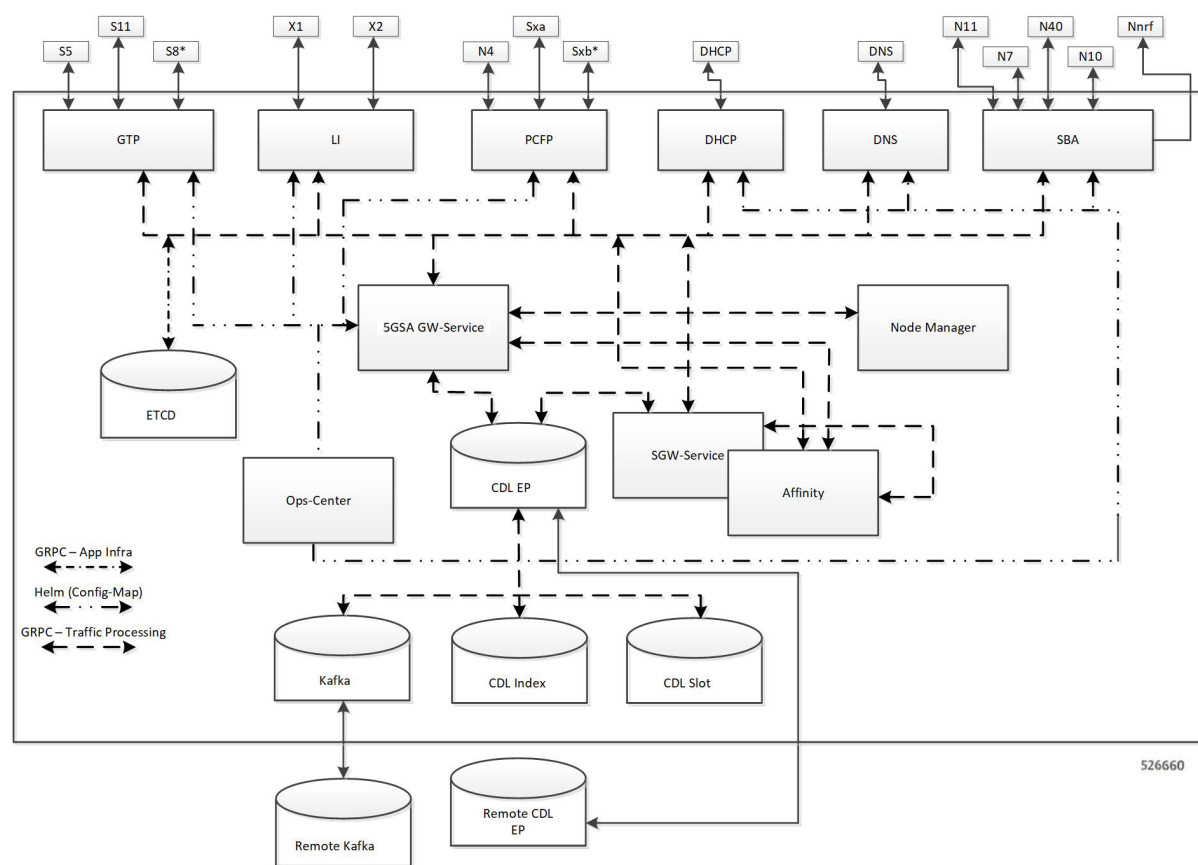
Figure 6: Kubernetes Deployment
