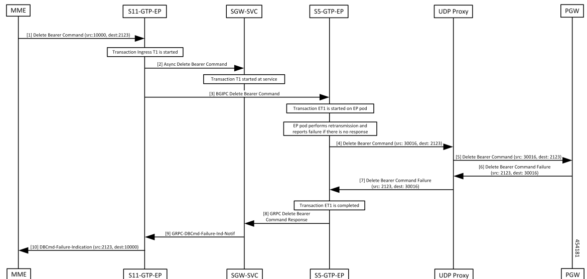
Figure 3: DBC Failure Handling Call Flow
