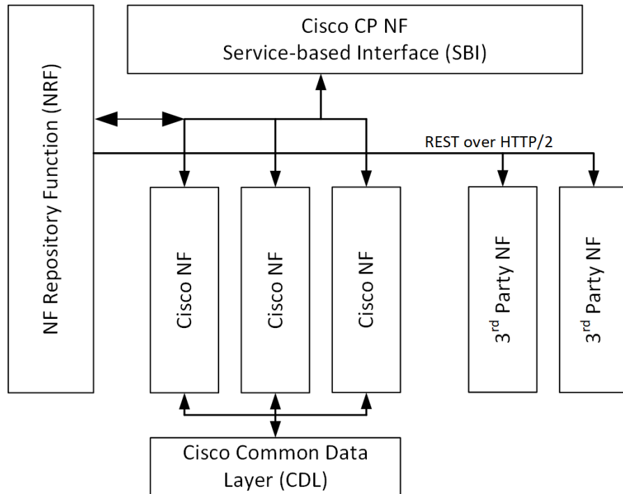
Figure 4: Cisco CP NF Service-based Architecture Support
