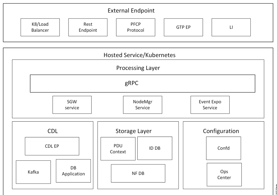
Figure 13: Communication Workflow of Pods
