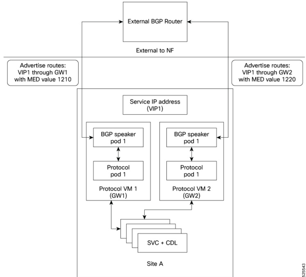
Figure 110: Dynamic Routing for Incoming Traffic in the Active-standby Topology
