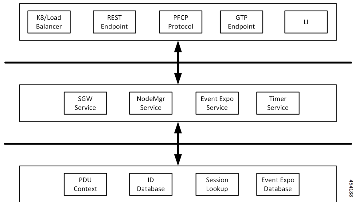
Figure 5: cnSGW-C Architecture
