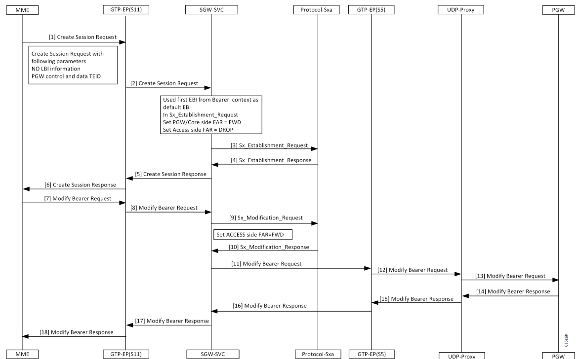
Figure 70: GnGp to LTE Handover with OI Indicator Unset Call Flow
