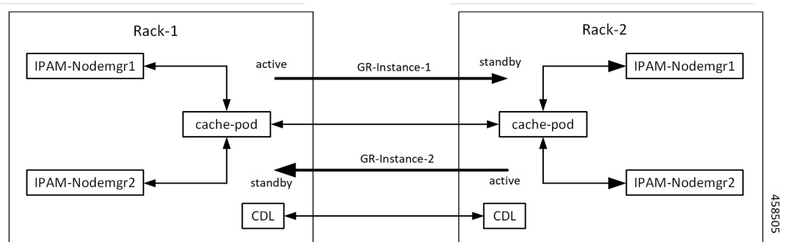
Figure 111: IPAM
