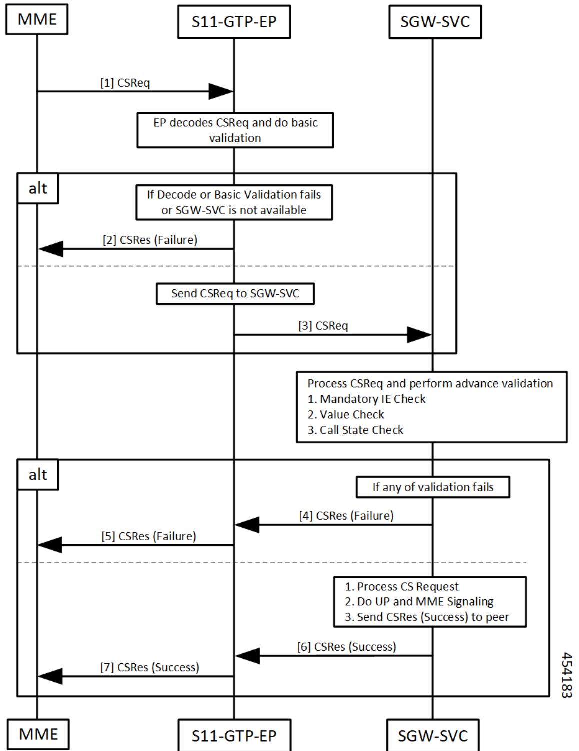
Figure 55: Basic and Advance Validation - S11 Call Flow
