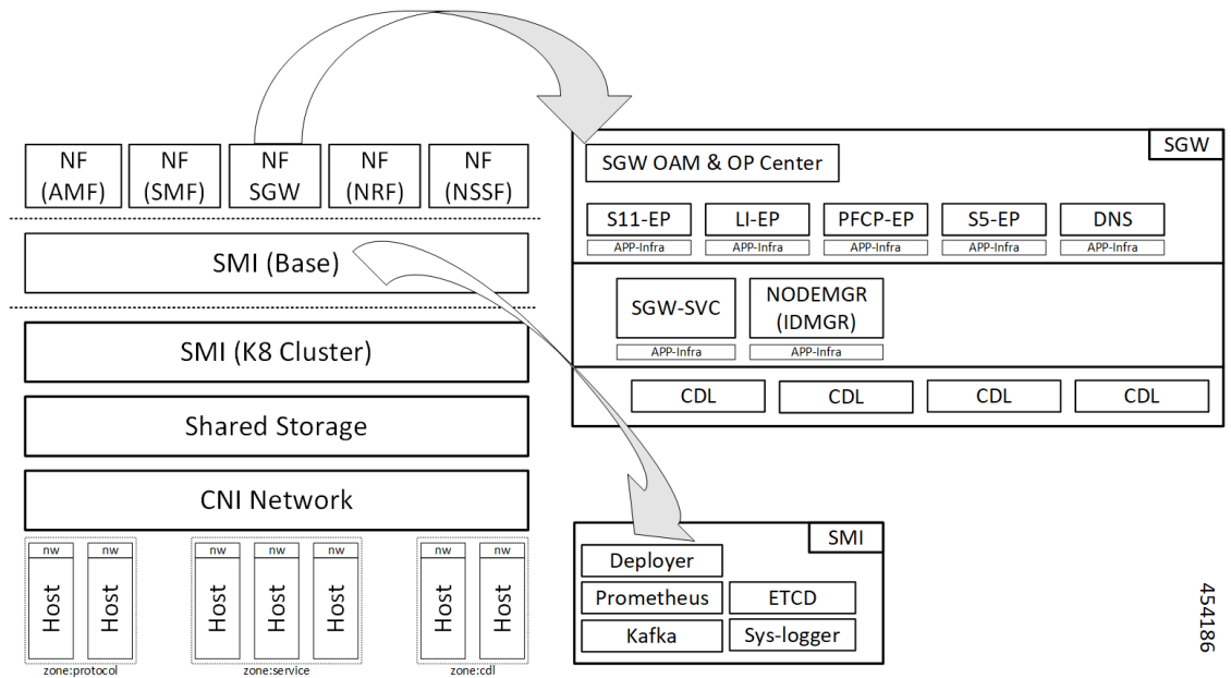
Figure 6: cnSGW-C Deployment
