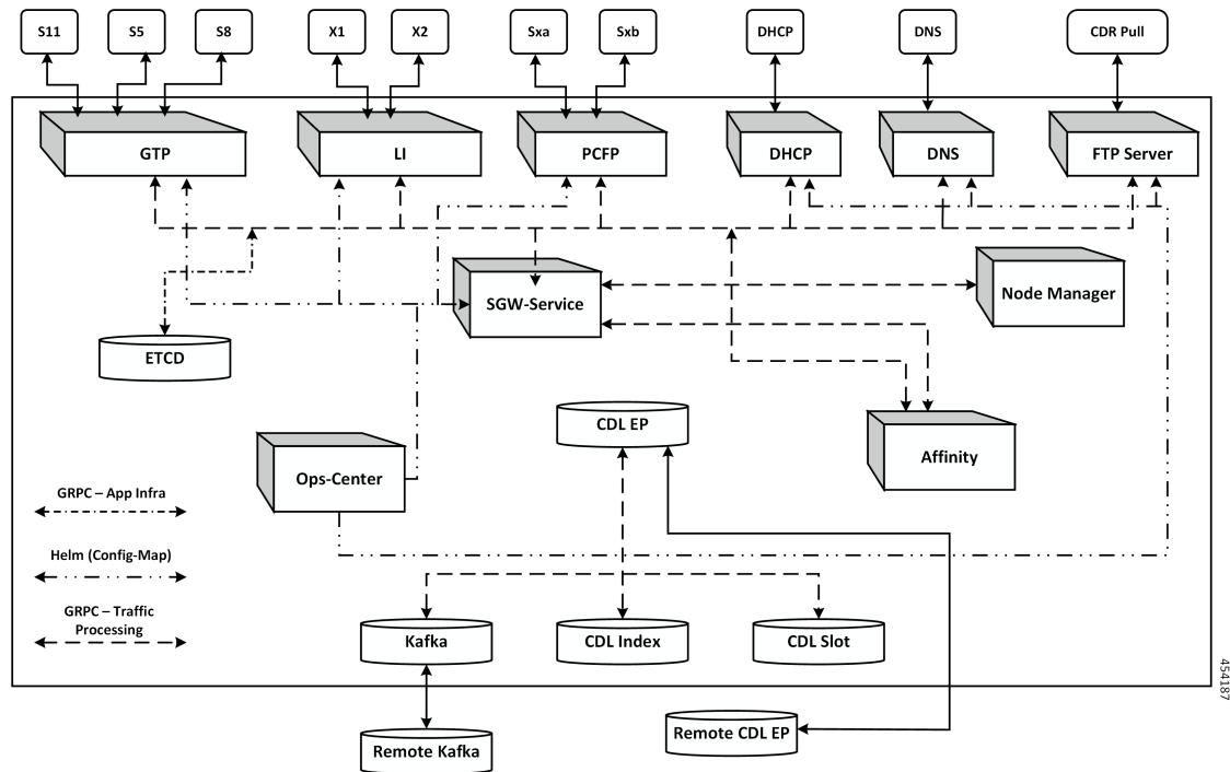
Figure 3: cnSGW-C HELM Chart
