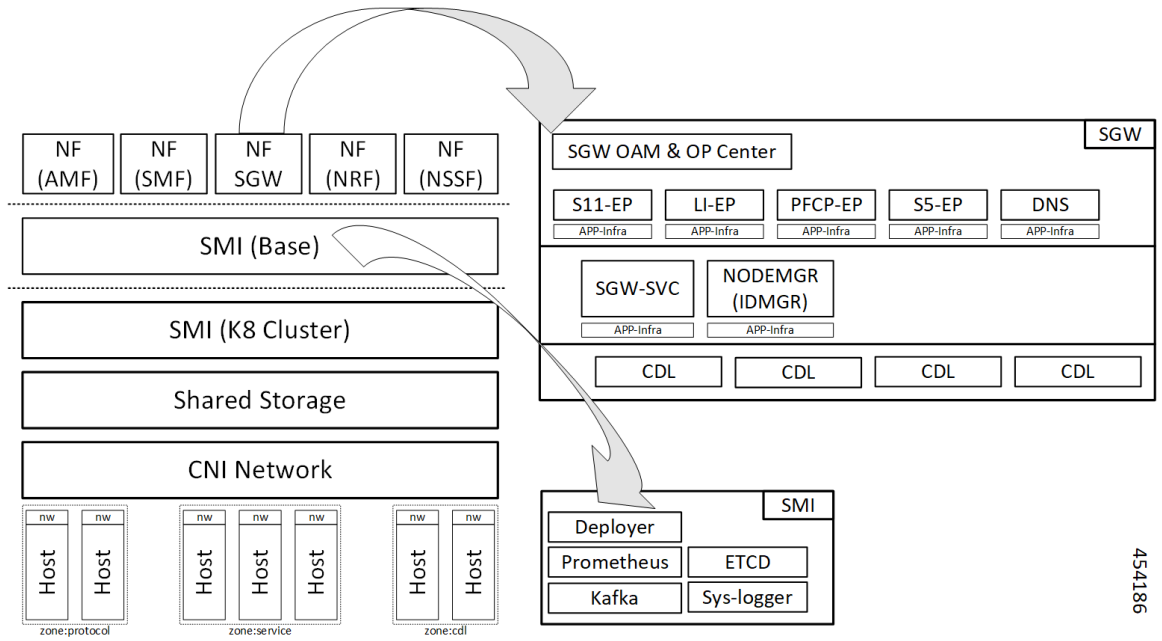
Figure 2: cnSGW-C Deployment
