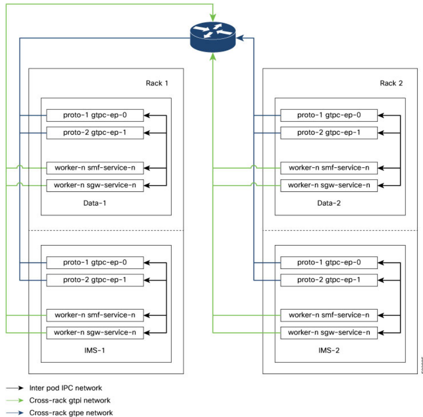
Figure 107: SGW-GTPC Inter-rack IPC
