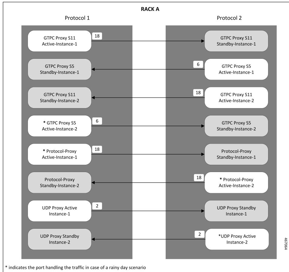
Figure 106: GTPC Interface Split pod layout
