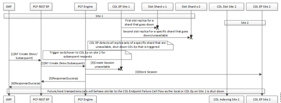
Figure 4: Slot Failure Call Flow Description
