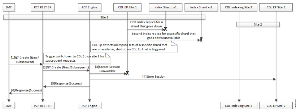
Figure 3: Indexing Shard Failure Call Flow Description
