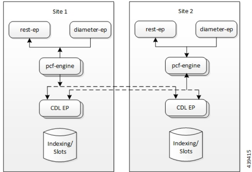
Figure 1: CDL Datastore Architecture
