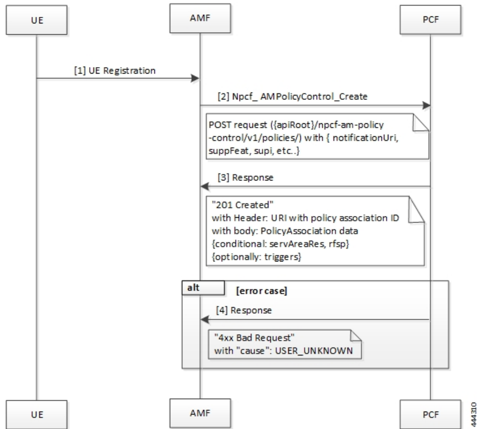
Figure 2: Create Policy Association Call Flow
