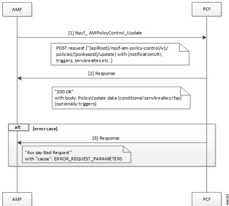
Figure 3: Update a Policy Association Call Flow
