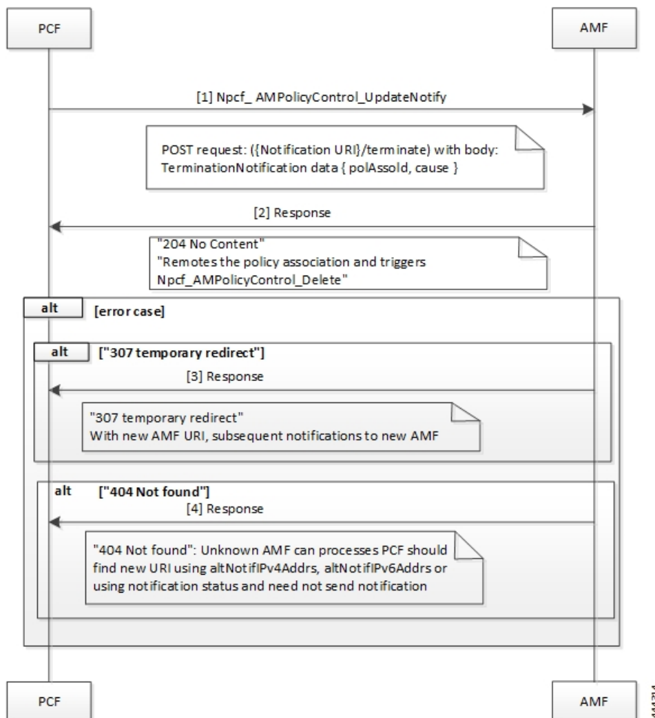
Figure 5: Terminate Policy Association Call Flow
