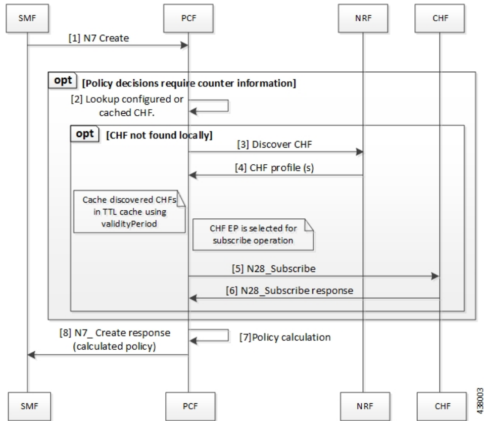
Figure 2: N28 Subscribe (N7 Create) Call Flow
