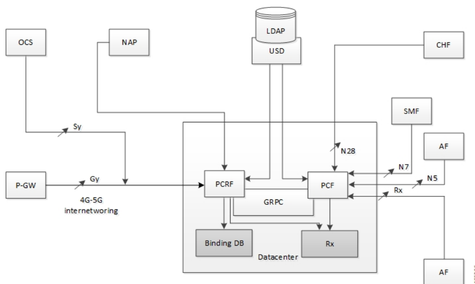
Figure 2: PCF Deployment
