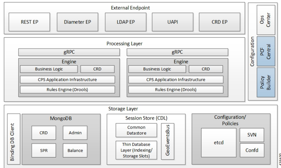
Figure 1: PCF Architecture
