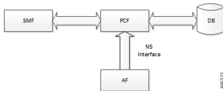
Figure 1: NF Interactions
