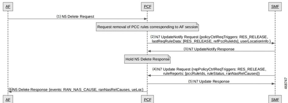
Figure 55: Deletion of Application Session with AF Call Flow
