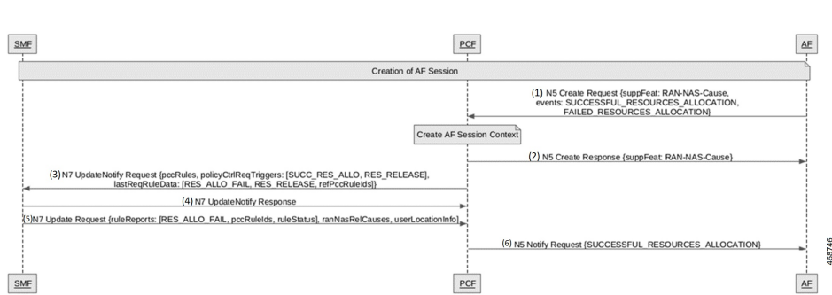
Figure 54: PCC Rule Installation and Modification Failures Call Flow
