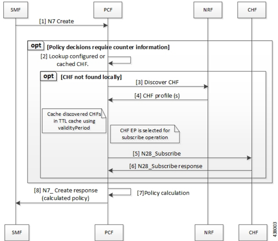
Figure 39: N28 Subscribe (N7 Create) Call Flow
