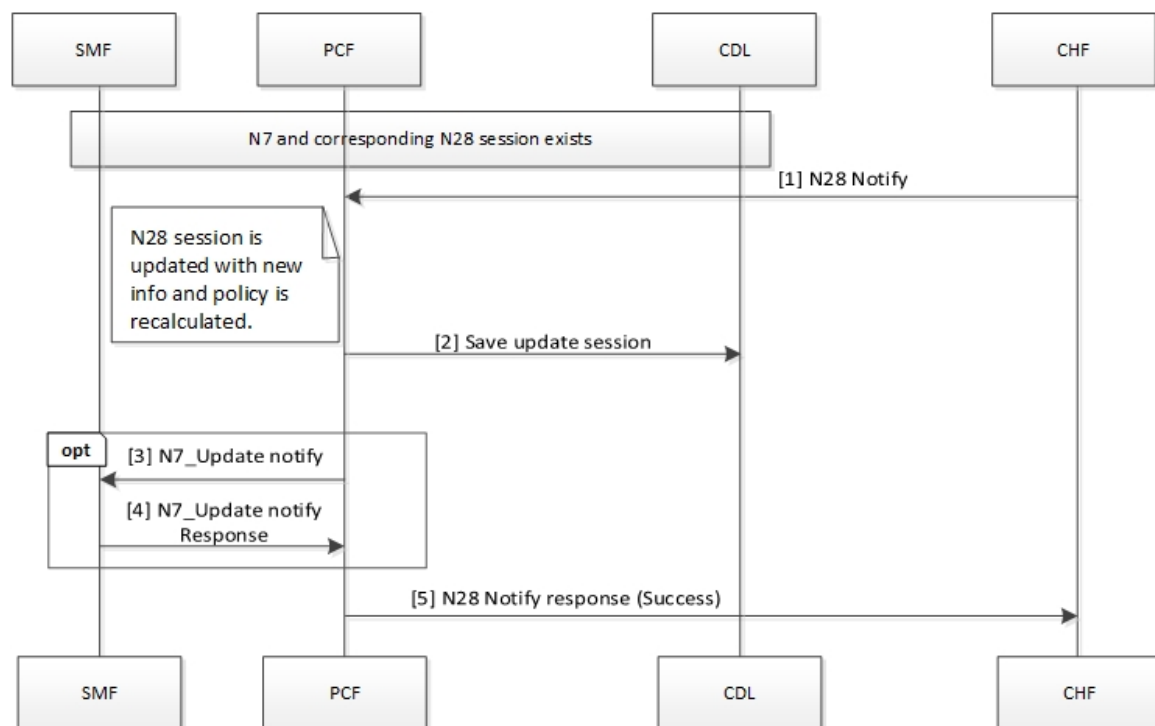
Figure 30: N28 Notify
