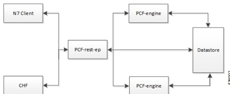
Figure 27: N28 Interface
