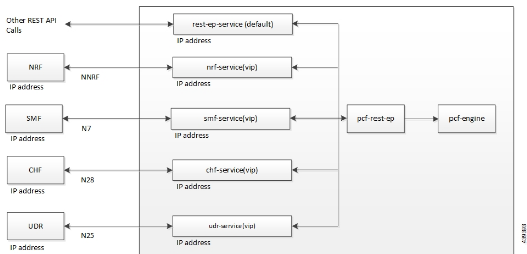
Figure 24: Multiple VIPs
