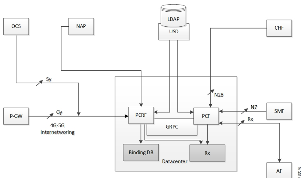
Figure 6: PCF Deployment
