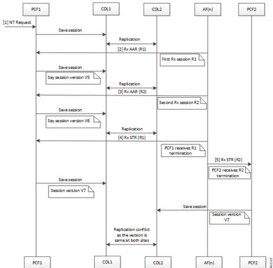
Figure 13: Local and Remote Sites Receive Rx_STR Without Any Time Gap Call Flow
