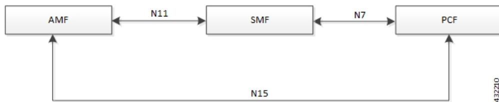
Figure 32: Interfaces in a Non-Roaming 5G System Architecture
