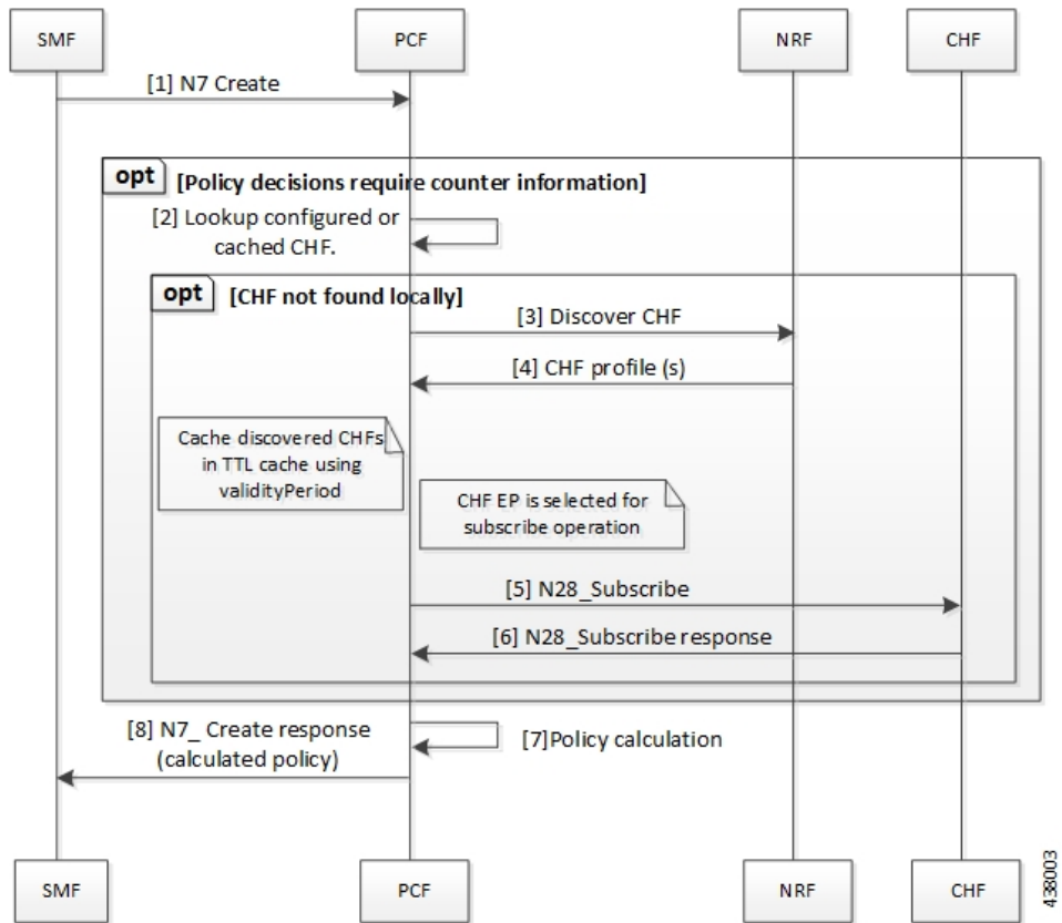
Figure 25: N28 Subscribe (N7 Create)
