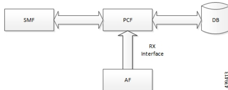
Figure 39: NF Interactions
