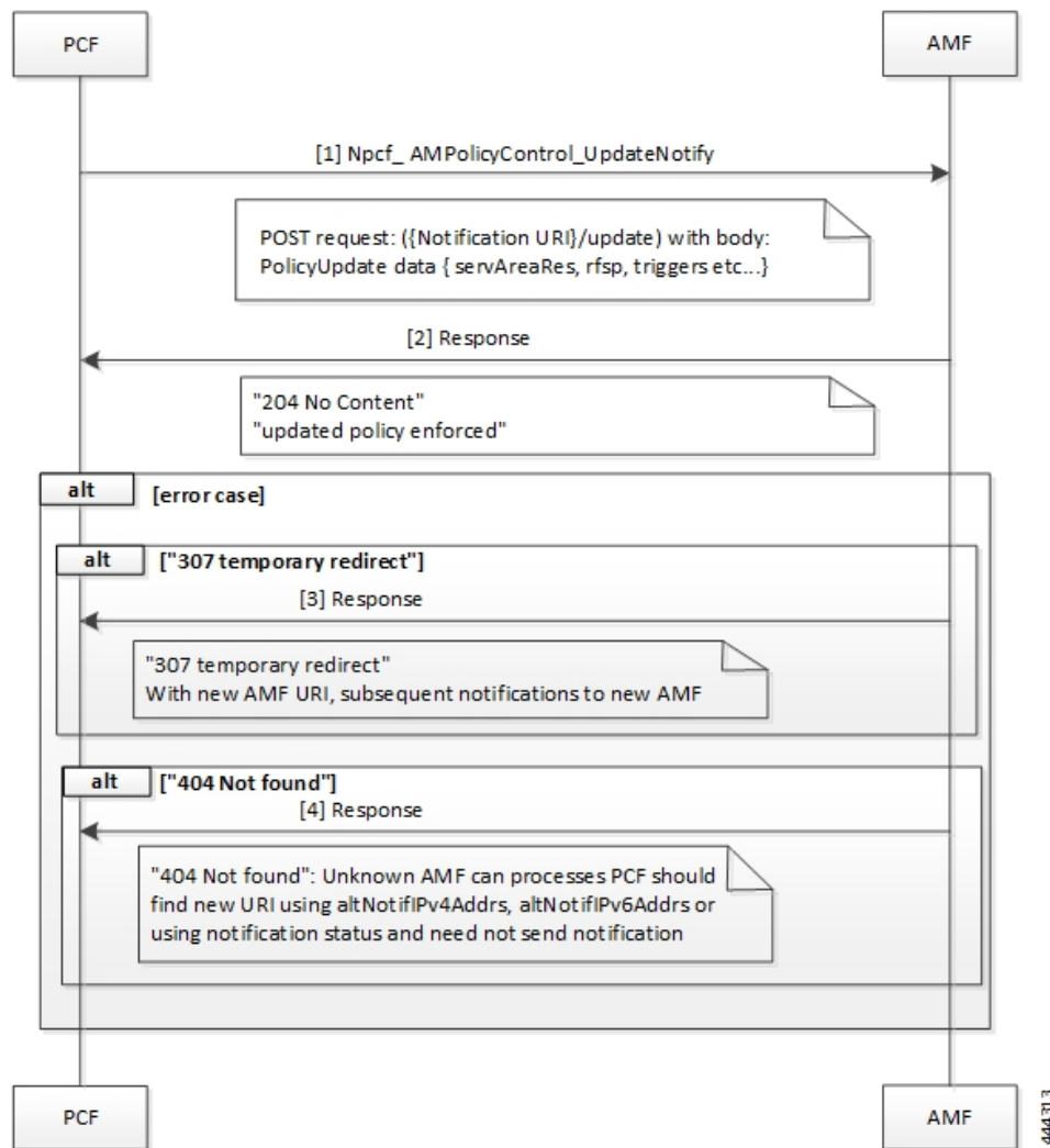
Figure 37: Update Notification Call Flow
