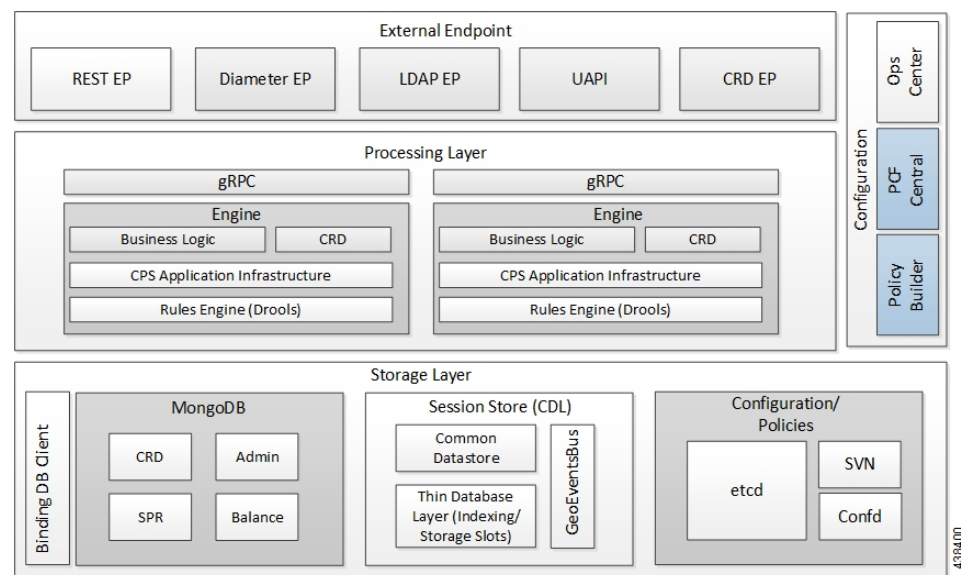
Figure 1: PCF Architecture
