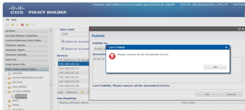
Figure 22: Unresolved error
