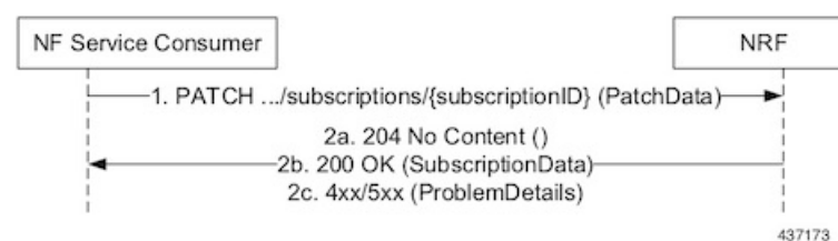
Figure 10: Subscription (PATCH) Call Flow
