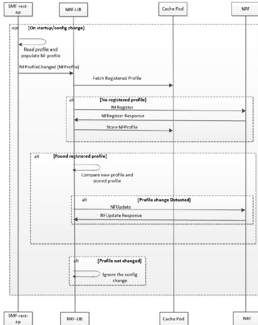
Figure 15: NF Registration and NF Update Call Flow
