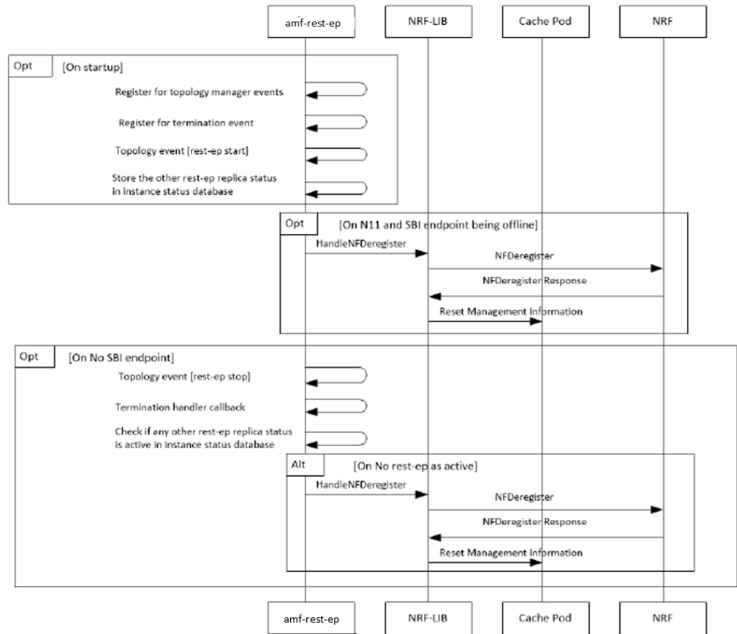
Figure 4: NF Deregistration Trigger Events Call Flow
