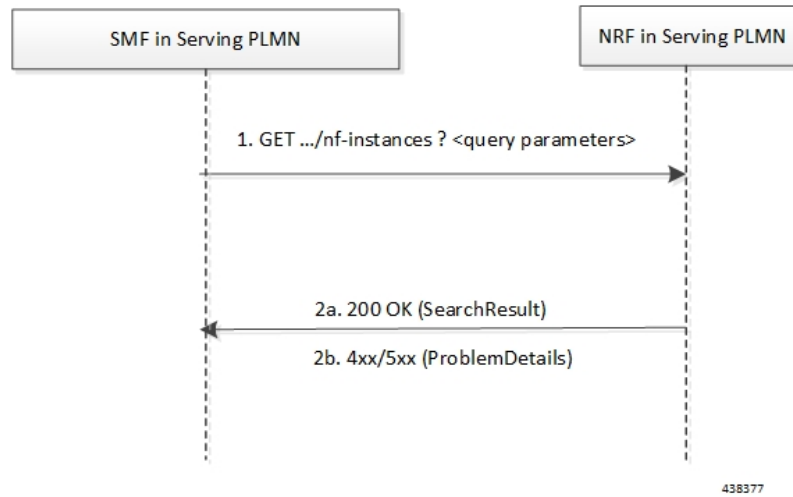
Figure 18: Service Discovery Request Call Flow
