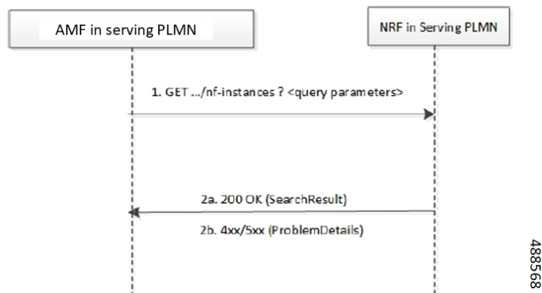
Figure 16: Service Discovery Request Call Flow
