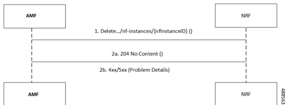
Figure 1: NRF Deregistration Call Flow
