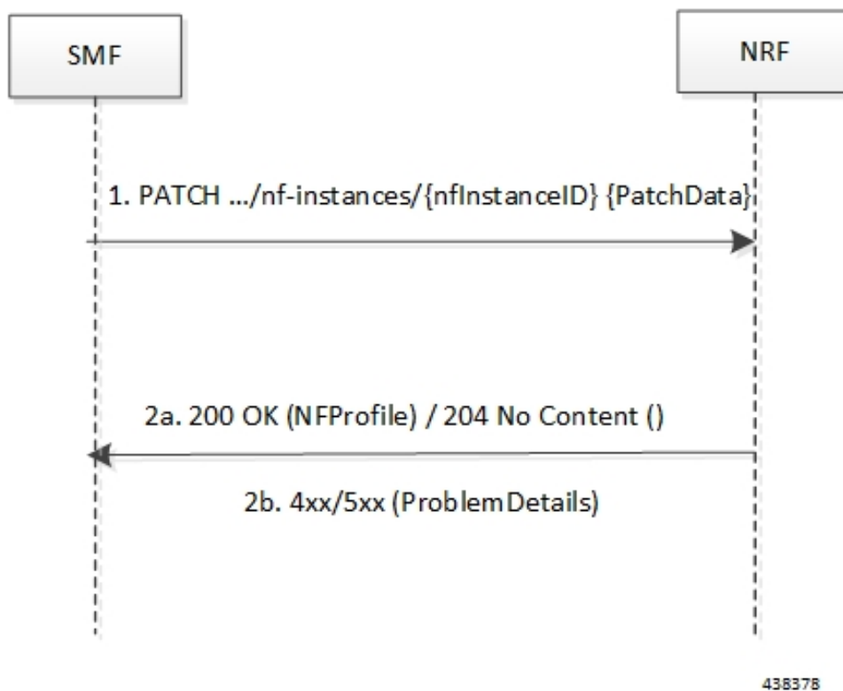
Figure 9: NF Heartbeat Call Flow
