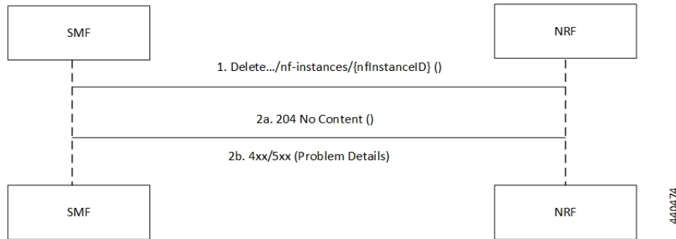
Figure 3: NRF Deregistration Call Flow
