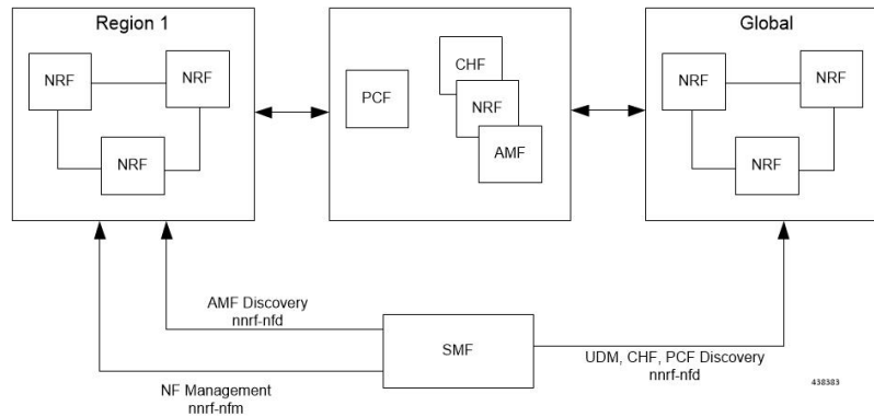
Figure 21: NRF Deployment
