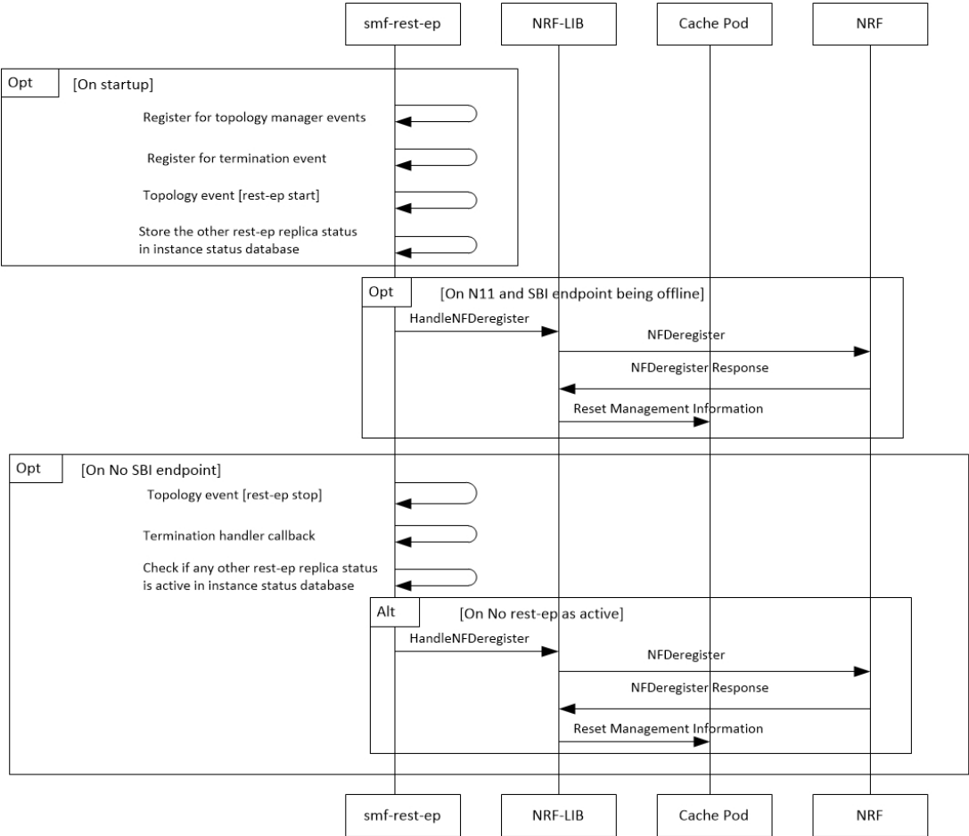
Figure 5: NF Deregistration Trigger Events Call Flow
