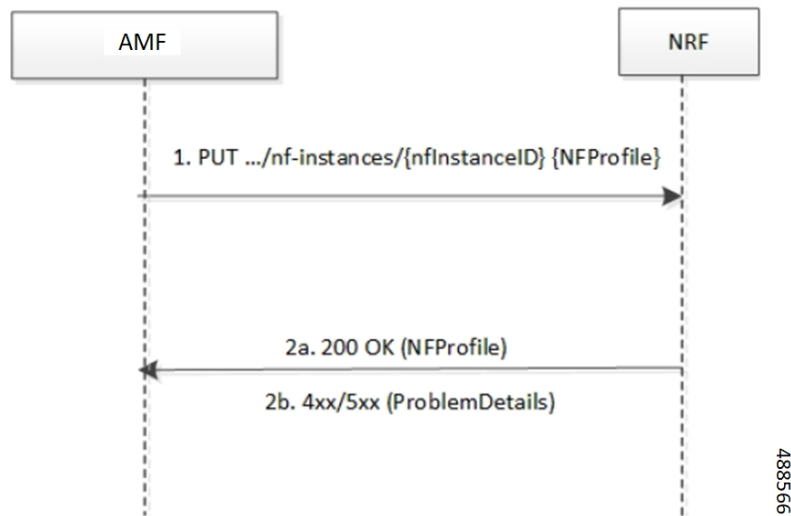
Figure 14: NF Profile Complete Replacement
