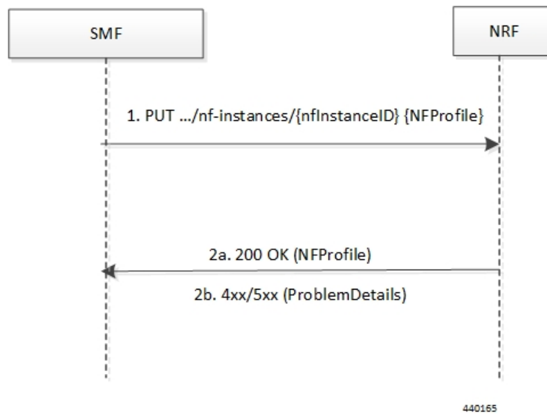
Figure 14: NF Profile Complete Replacement
