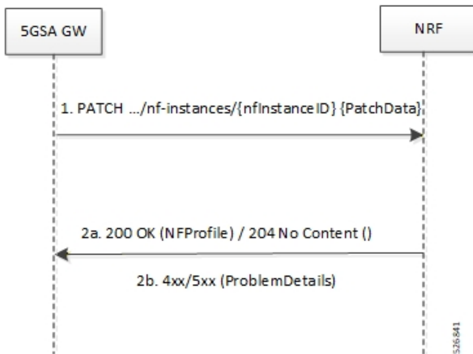
Figure 9: NF Heartbeat Call Flow
