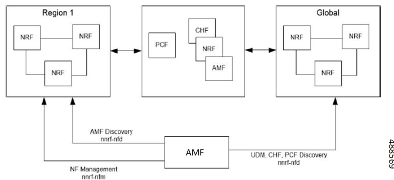
Figure 19: NRF Deployment
