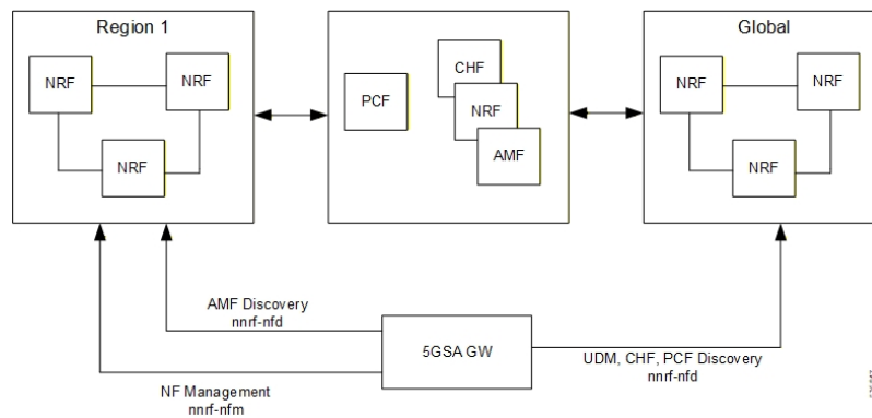
Figure 21: NRF Deployment
