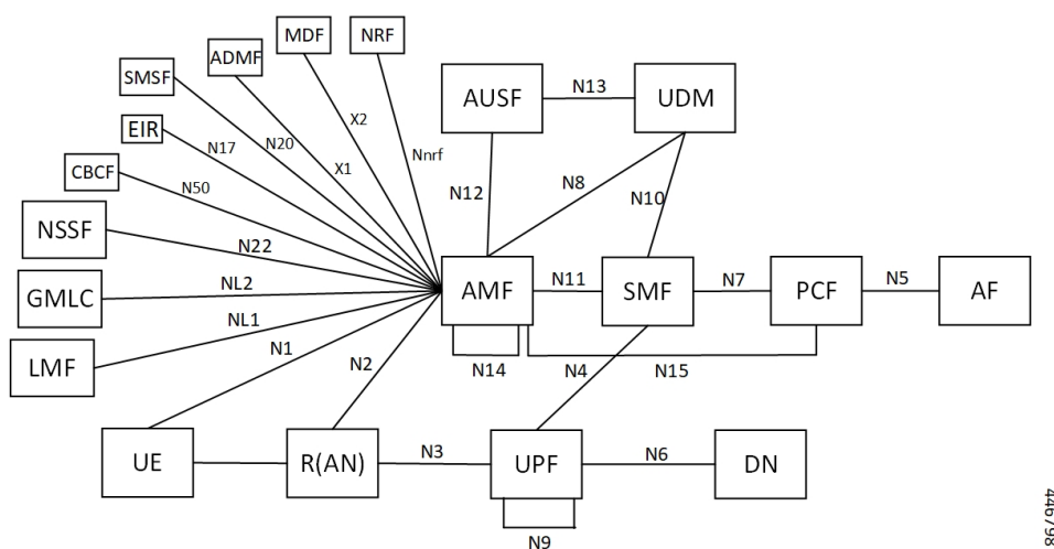
Figure 5: Interfaces
